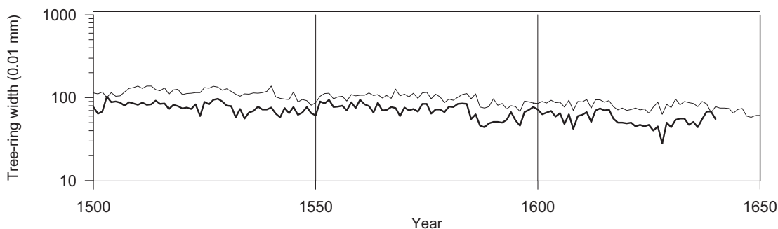
Figure 6. The tree-ring sequence of the violin 2 (bold curve) with the last ring dated to 1640, and the chronology 250mk_01 of Steiner's instruments (entire span 1336-1686) (thin curve)
