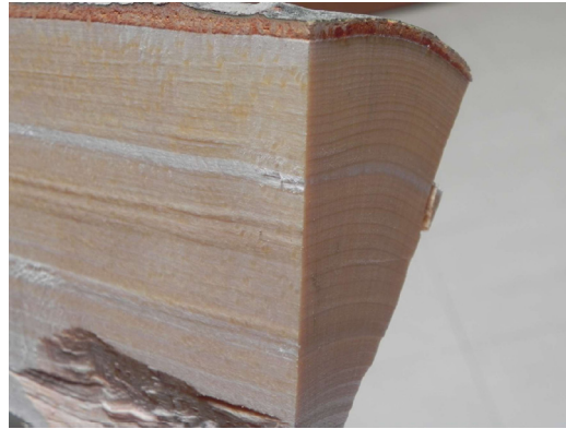
Fig. 12: Tension wood
