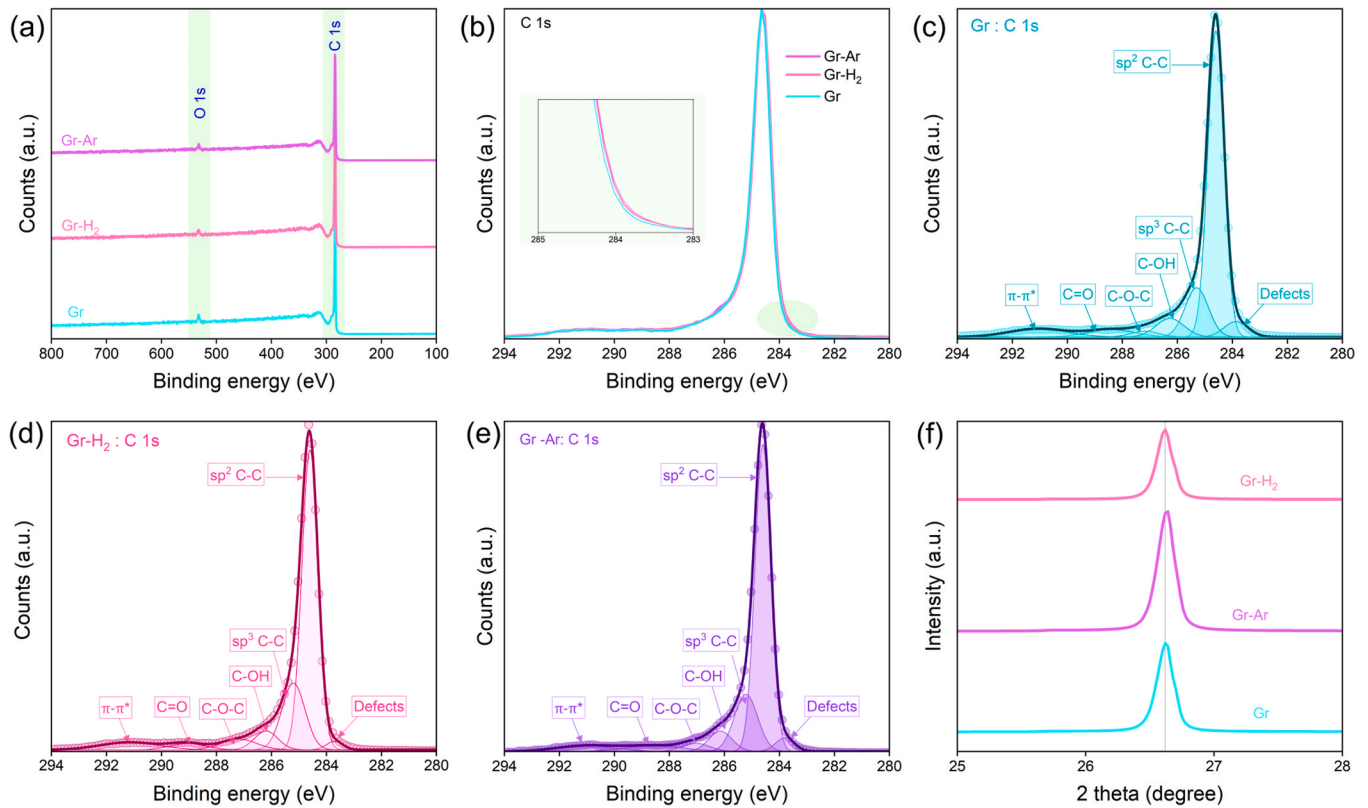
Fig. 3. (a) XPS survey spectra of graphite and plasma tailored graphite flakes; (b) Comparison of high-resolution C 1s spectra with the noticeable changes in the defect region in the inset; deconvoluted C 1s spectra of (c) graphite, (d) H 2 -plasma treated graphite and (e) Ar-plasma treated graphite; (f) XRD pattern of pure and plasma engineered graphite around the characteristic (002) diffraction peak.
