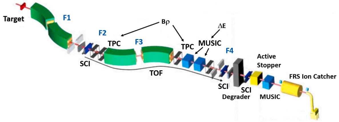
Fig. 1. Schematic view of the experimental setup of FRS from the target to the final focal plane. The F2 and F4 focal planes host the detectors used for the particle identification. The detectors at F4, downstream of the degrader, are used to monitor the implantation in either the active stopper or in the FRS Ion Catcher.
