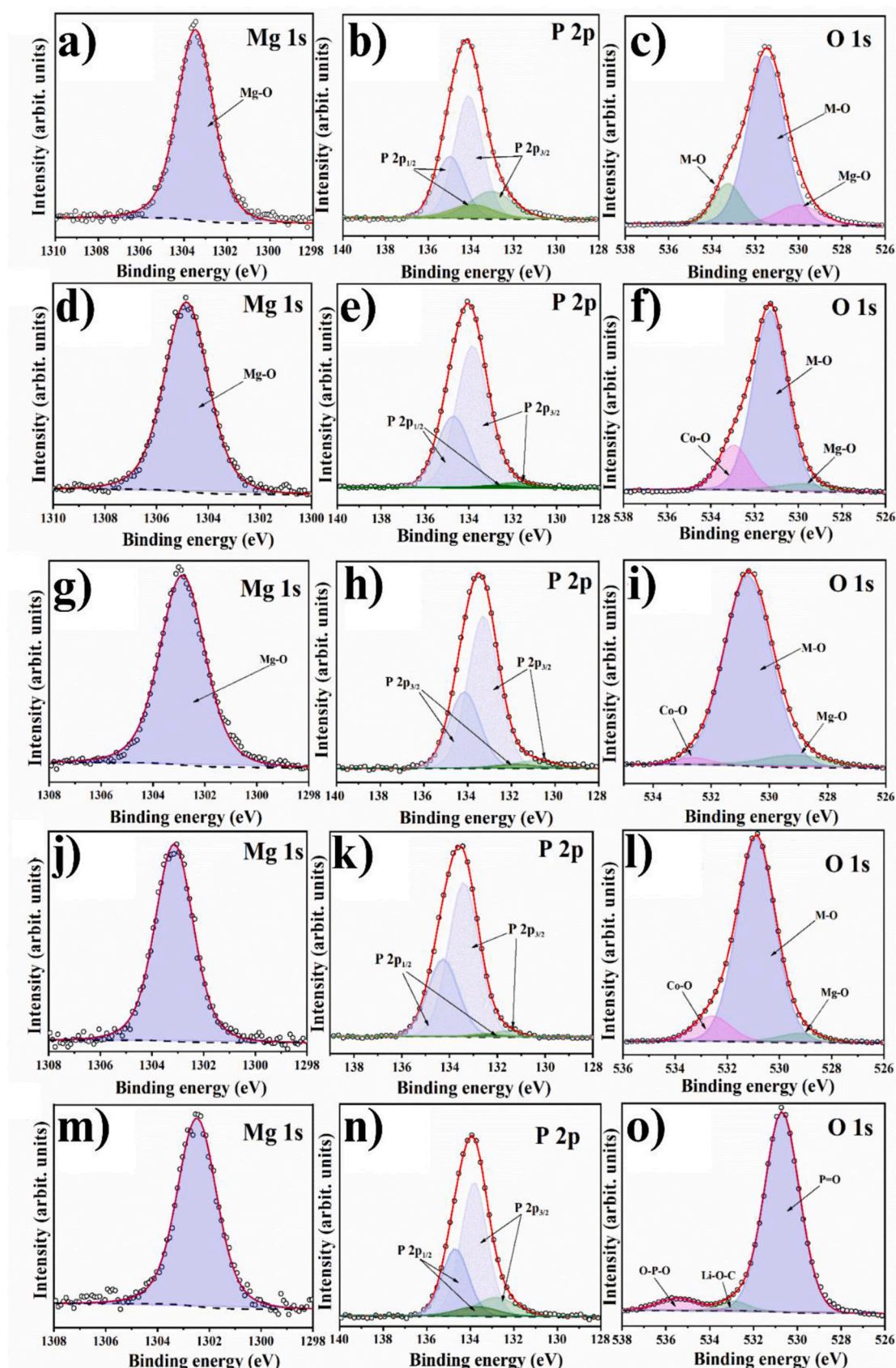
Fig. 6. XPS of the Sample 1 (a, b, c); Sample 2 (d, e, f); Sample 3 (g, h, i); Sample 4 (j, k, l) and Sample 5 (m, n, o) for the center level spectra of the elements Mg 1s, P 2p and O 1s.
