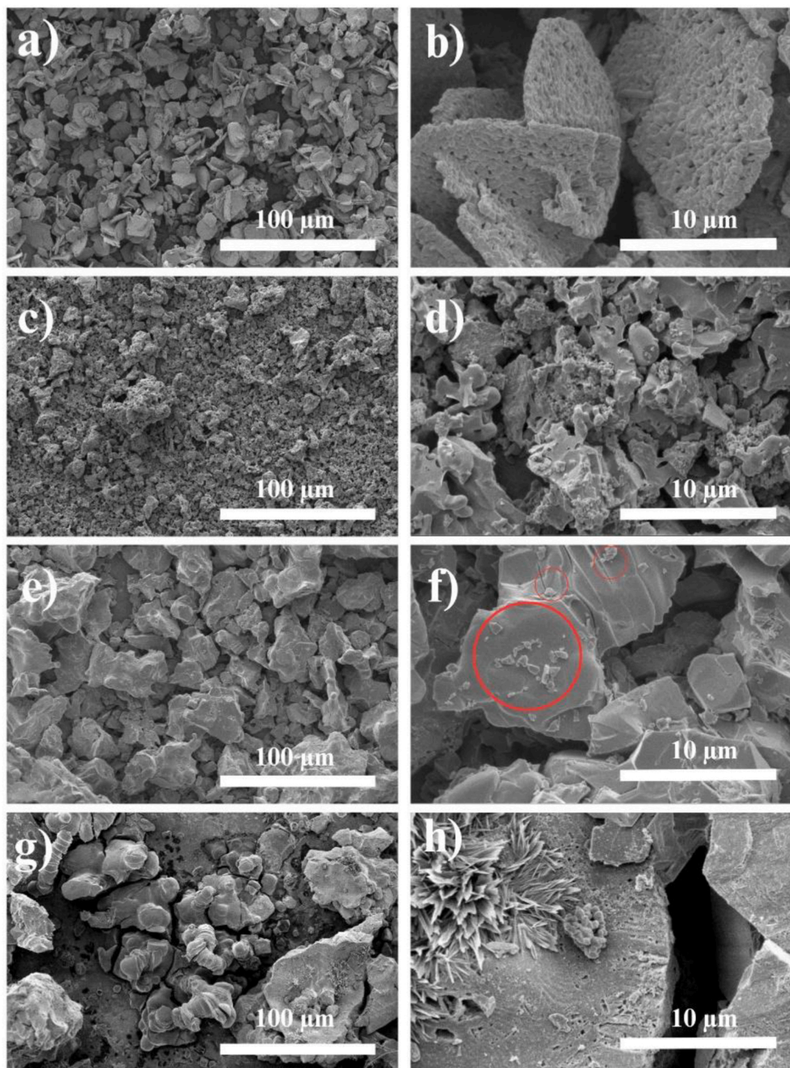
Fig. 4. Micrographs of the pigments (a-b) Sample 2; (c-d) Sample 3; (e-f) Sample 4 and (g-h) Sample 5.
