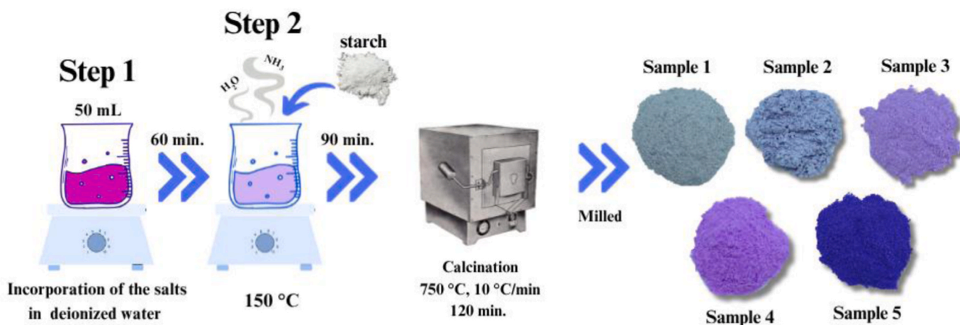
Fig. 1. Scheme for synthesizing magnesium phosphate and cobalt pigments based on starch.
