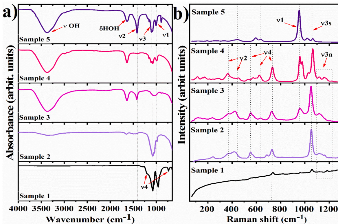
Fig. 8. FTIR (a) and Raman (b) spectra of the metallophosphates pigments.
