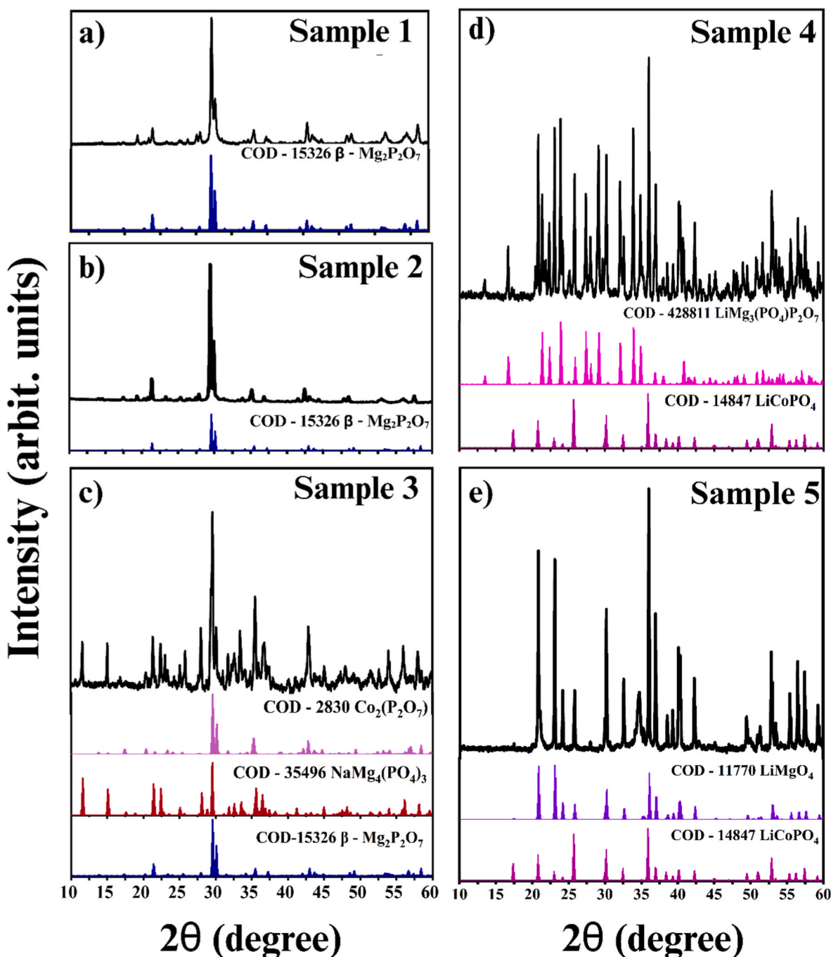
Fig. 5. X-ray diffractograms for pigments a) Sample 1; b) Sample 2 c) Sample 3; d) Sample 4 and e) Sample 5.
