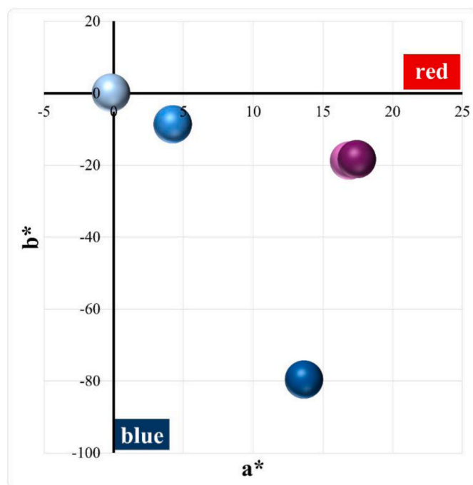
Fig. 11. Graph of colorimetric parameters red (+a) versus blue (-b).
