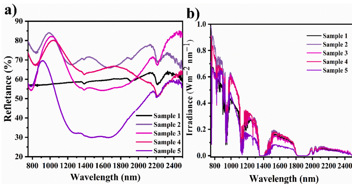
Fig. 10. (a) Diffuse reflectance spectra of the powdered pigments synthesized, and (b) NIR solar reflectance spectra of the powdered pigments adjusted to the standard solar spectrum.
