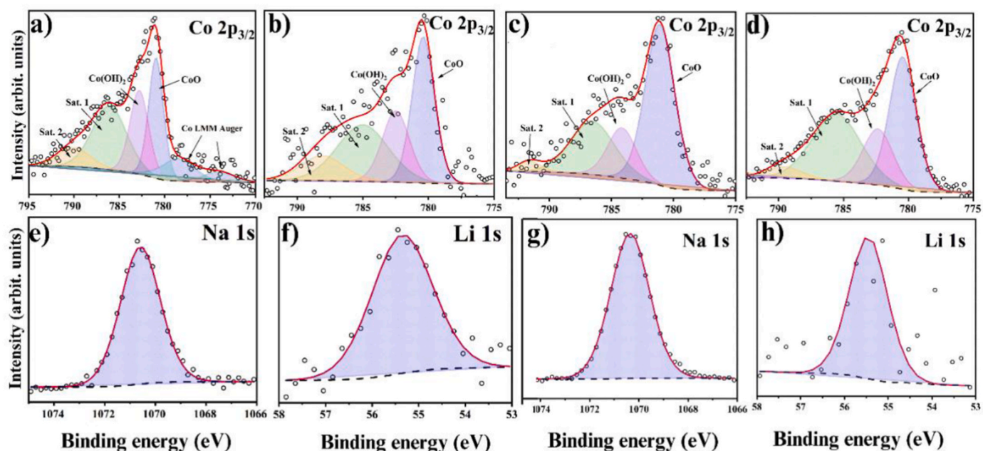
Fig. 7. XPS of the pigments Sample 2 (a), Sample 3 (b), Sample 4 (c), and Sample 5 (d) for the center level spectra element Co 2p. XPS and Sample 3 (e); Sample 4 (f), Sample 5 (g and h), for the center level spectra of the elements Na 1s and Li 1s.
