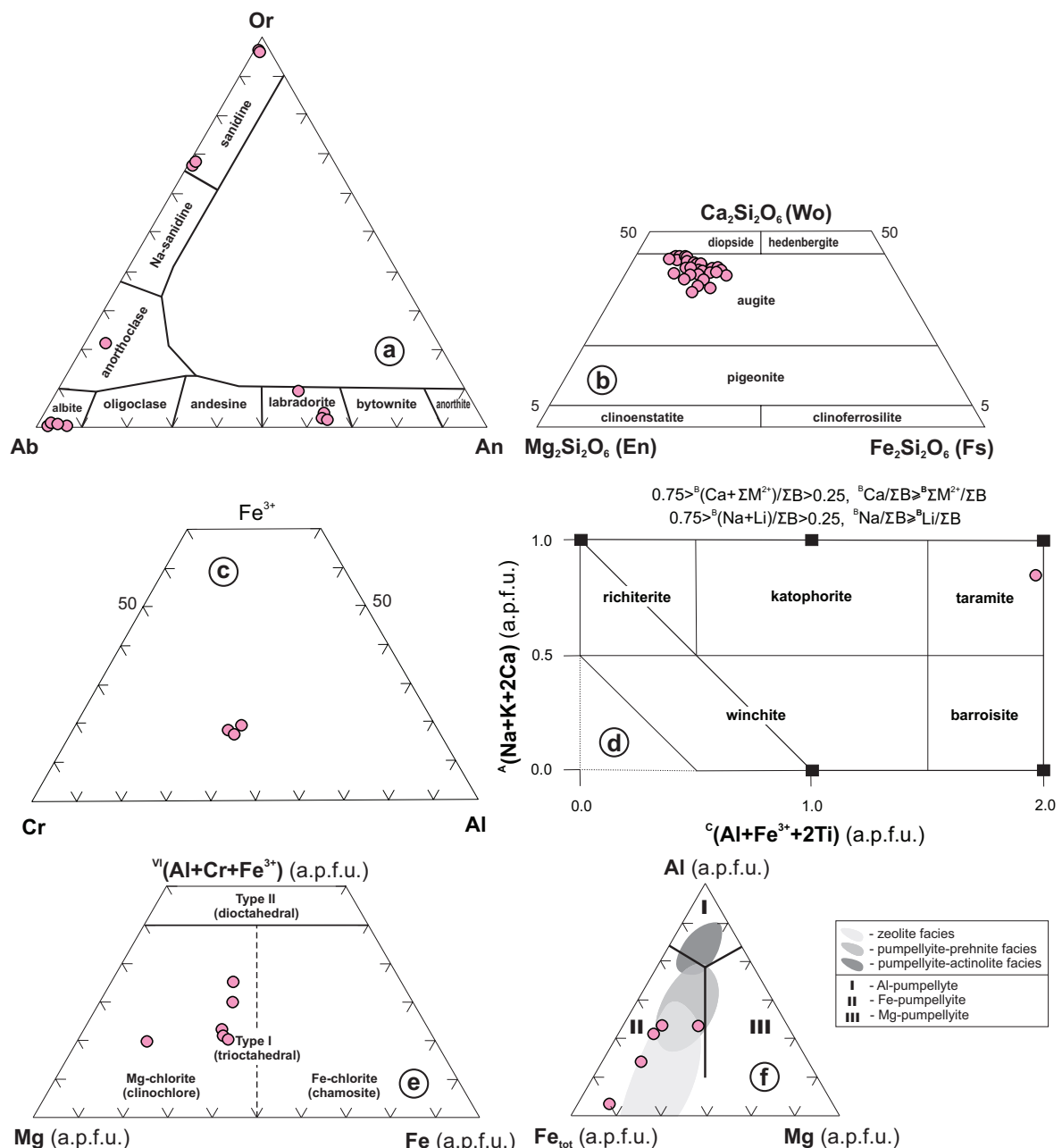
Fig. 6. Classification diagrams for (a) feldspar (Ab–An–Or plot; Deer et al. 1992; Dana et al. 1993), (b) pyroxene (En–Wo–Fs ( \text{Mg}_2\text{Si}_2\text{O}_6 – \text{Ca}_2\text{Si}_2\text{O}_6 – \text{Fe}_2\text{Si}_2\text{O}_6 ) plot; Morimoto 1988), (c) spinel (trivalent Cr–Al– \text{Fe}^{3+} ternary cation plot; from Leake et al. 1997 and Hawthorne et al. 2012), (d) amphibole ( \text{Al}^{IV}/(\text{Na}+\text{K})^A plot; from Leake et al. 1997 and Hawthorne et al. 2012), (e) chlorite [ \text{Mg} – \text{Fe} – \text{Al}^{VI}/(\text{Al}+\text{Cr}+\text{Fe}^{3+}) plot; Zane & Weiss 1998] and (f) pumpellyite ( \text{Fe}_{\text{tot}} – \text{Mg} – \text{Al} plot; Coombs et al. 1976) from the Middle Triassic calc-alkaline basaltic rocks from the Mt. Ivanščica. Compositional fields for pumpellyite from the East Taiwan Ophiolite basalts (zeolite facies), basalts from the Olympic Peninsula (prehnite–pumpellyite facies) and basalts from the Tavayannaz Formation (upper prehnite–pumpellyite and pumpellyite–actinolite facies) are taken from Coombs et al. (1976) and Rahn et al. (1994), respectively.
