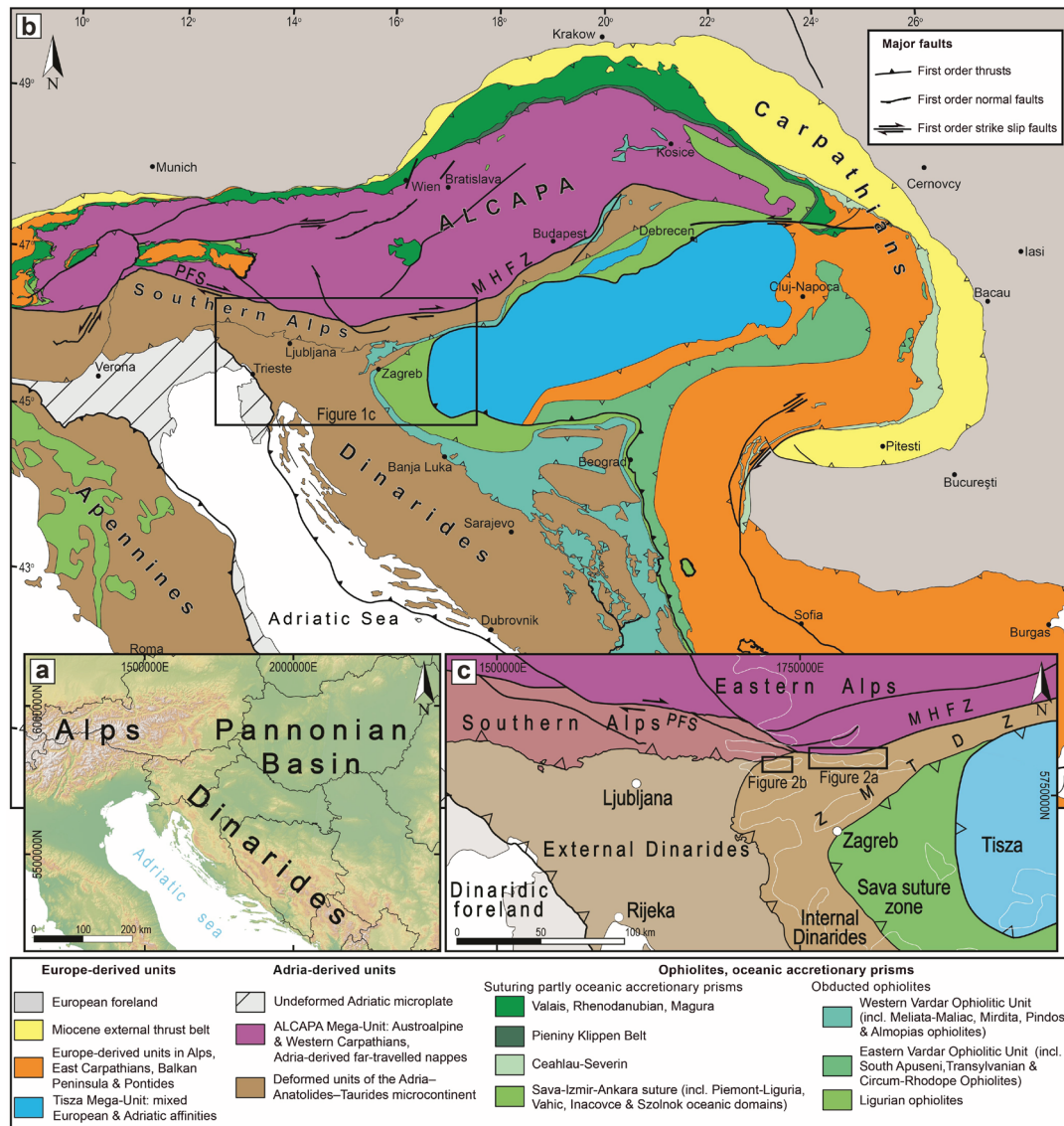
Fig. 1. (a) Topographic map of Alps, Dinarides, and Pannonian Basin. (b) Simplified tectonic map of Schmid et al. (2020) showing major tectonic units of the Dinarides, Alps, Carpathians, and Tisza. (c) Detail from the figure 1b, modified according to Vukovski et al. (2024, 2026). The investigated areas (marked with two black rectangles) occupy a position at the northernmost part of the Dinarides close to the tectonic units of the Alps to the north, in the southwestern part of the Pannonian Basin (white outlines). ZMTDZ=Zagorje–Mid-Transdanubian Zone; PFS=Periadriatic Fault System; MHFZ=Mid-Hungarian Fault Zone.
