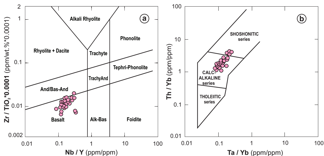
Fig. 7. (a) Nb/Y– Zr/TiO_2 \cdot 10^{-4} classification diagram (Pearce 1996) and (b) Ta/Yb–Th/Yb discrimination diagram (Müller et al. 1992) for the Middle Triassic calc-alkaline basaltic rocks from the Ivanščica, Strahinjščica, Desinić Gora, and Olimska Gora Mts.
