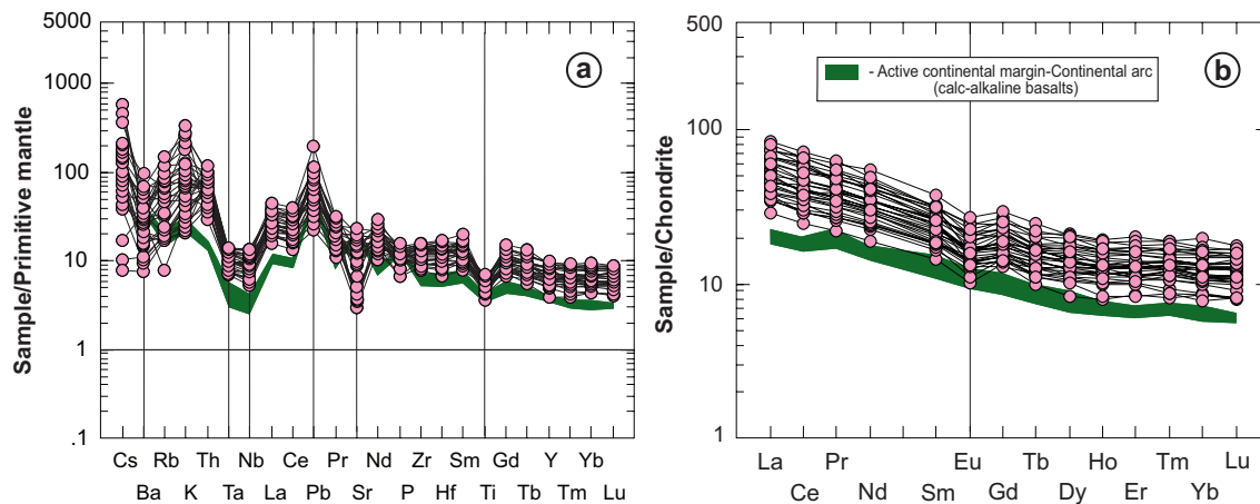
Fig. 8. (a) Primitive mantle-normalised multielement and (b) chondrite-normalised REE diagrams for the Middle Triassic calc-alkaline basaltic rocks from the Ivanščica, Strahinjščica, Desinić Gora, and Olimska Gora Mts. Normalisation values are from Sun & McDonough (1989). Patterns for average primitive calc-alkaline basalt from active continental margin-continental arc (Schmidt & Jagoutz 2017) are plotted for correlation constrains.
