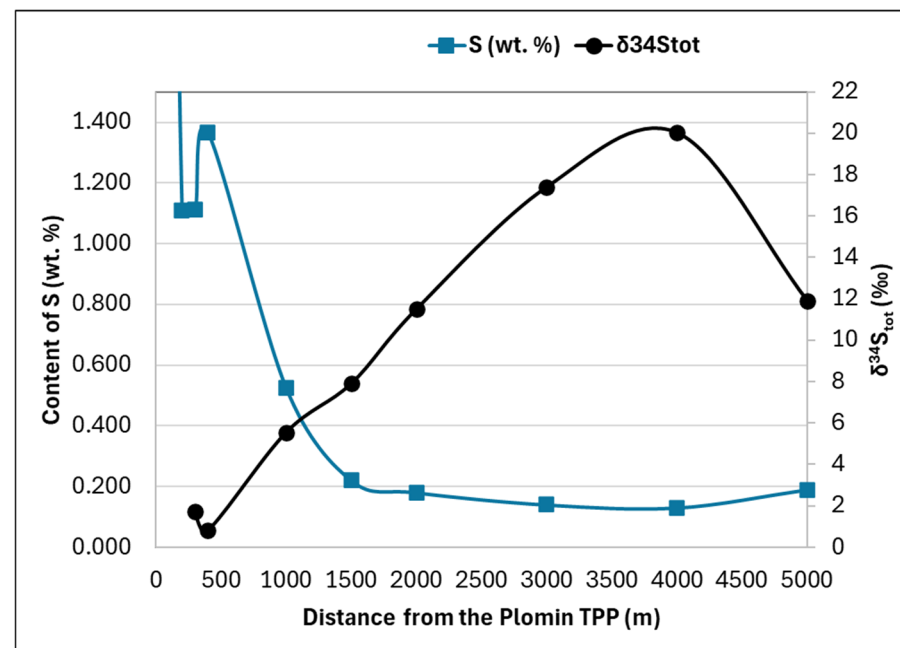
Figure 4. Relation between content and isotopic composition of S in soil and distance from the Plomin TPP.
