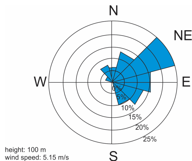
Figure 2. Wind rose showing the long-term (2008–2017) prevailing wind direction in the study area, derived from a regional wind atlas [26] based on multi-year meteorological observations. NE dominance reflects average conditions, not a unidirectional wind [26].
