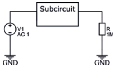
Figure 1: Measuring circuit setup
