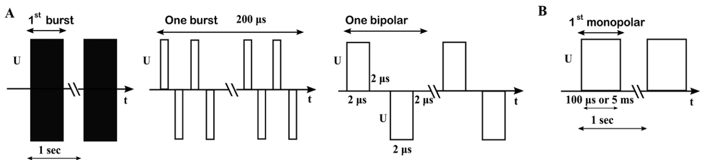
FIGURE 1. (A) 50 \times 50 HF pulses. From left to right: 50 bursts were applied with a repetition frequency of 1 Hz; one burst with 200 \mu s total pulse on time and consisted of 50 bipolar pulses; one bipolar pulse of amplitude U consisted of a 2 \mu s long positive pulse, and a 2 \mu s long negative pulse (both of voltage U ) with a 2 \mu s long interpulse delay. (B) 8 \times 100 \mu s or 8 \times 5 ms monopolar pulse of amplitude U and pulse duration of 100 \mu s or 5 ms were applied with a repetition frequency of 1 Hz
