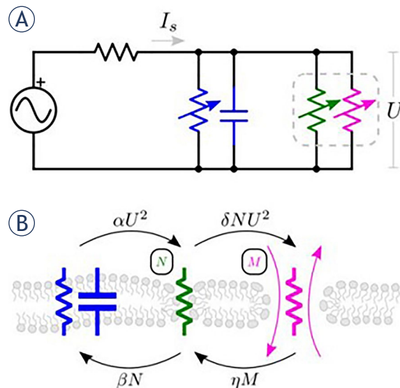
FIGURE 2. Schematic of the model that describes electroporation and molecular transport. (A) The equivalent circuit, which considers electroporation (membrane pore/defect formation) to be a two-step process, as depicted in (B). The blue capacitance and resistance represent the intact cell membrane. When the electric field is applied, the cell membrane becomes permeable first to small ions, indicating the first porous state (N) of the membrane represented by green resistance. Then the membrane becomes permeable to small molecules, indicating the second porous state (M) of the membrane represented by magenta resistance. Reproduced from Sweeney et al. 56 with permission.
