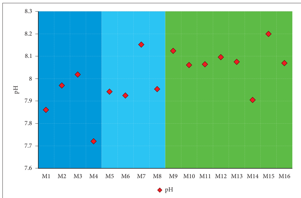
Figure 4: Average pH values at sample sites.
