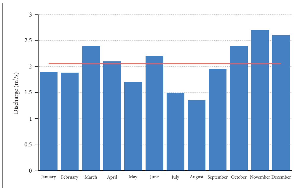
Figure 1: Hydrogram of Medja near Zagorje ob Savi for the period 1981–2010 (data source: ARSO 2021c).
