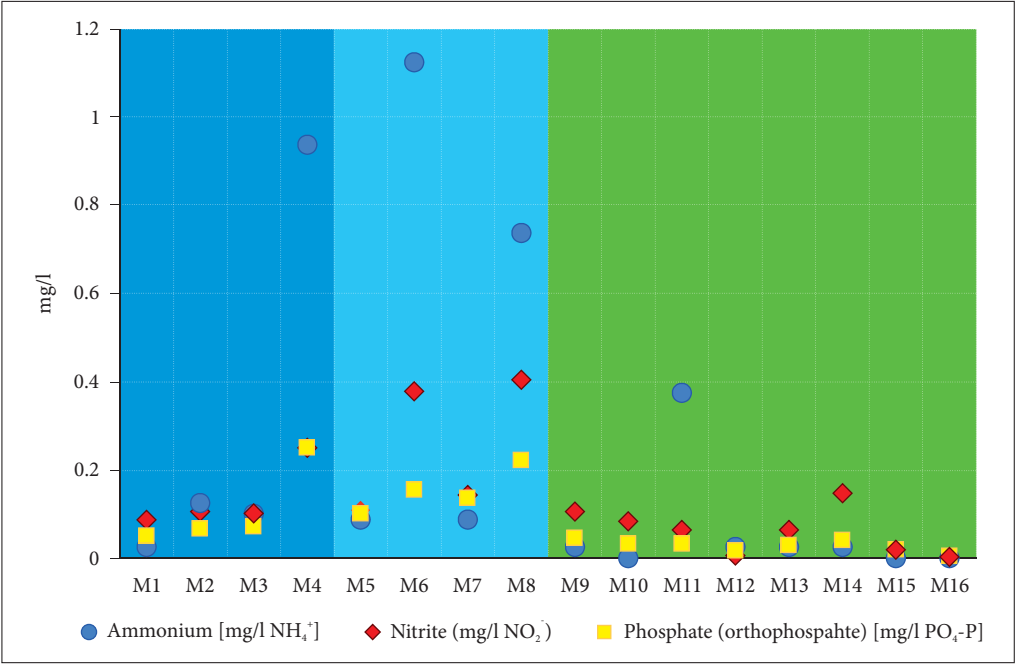
Figure 6: Average values of nitrite, ammonium and phosphate at the sample sites.
