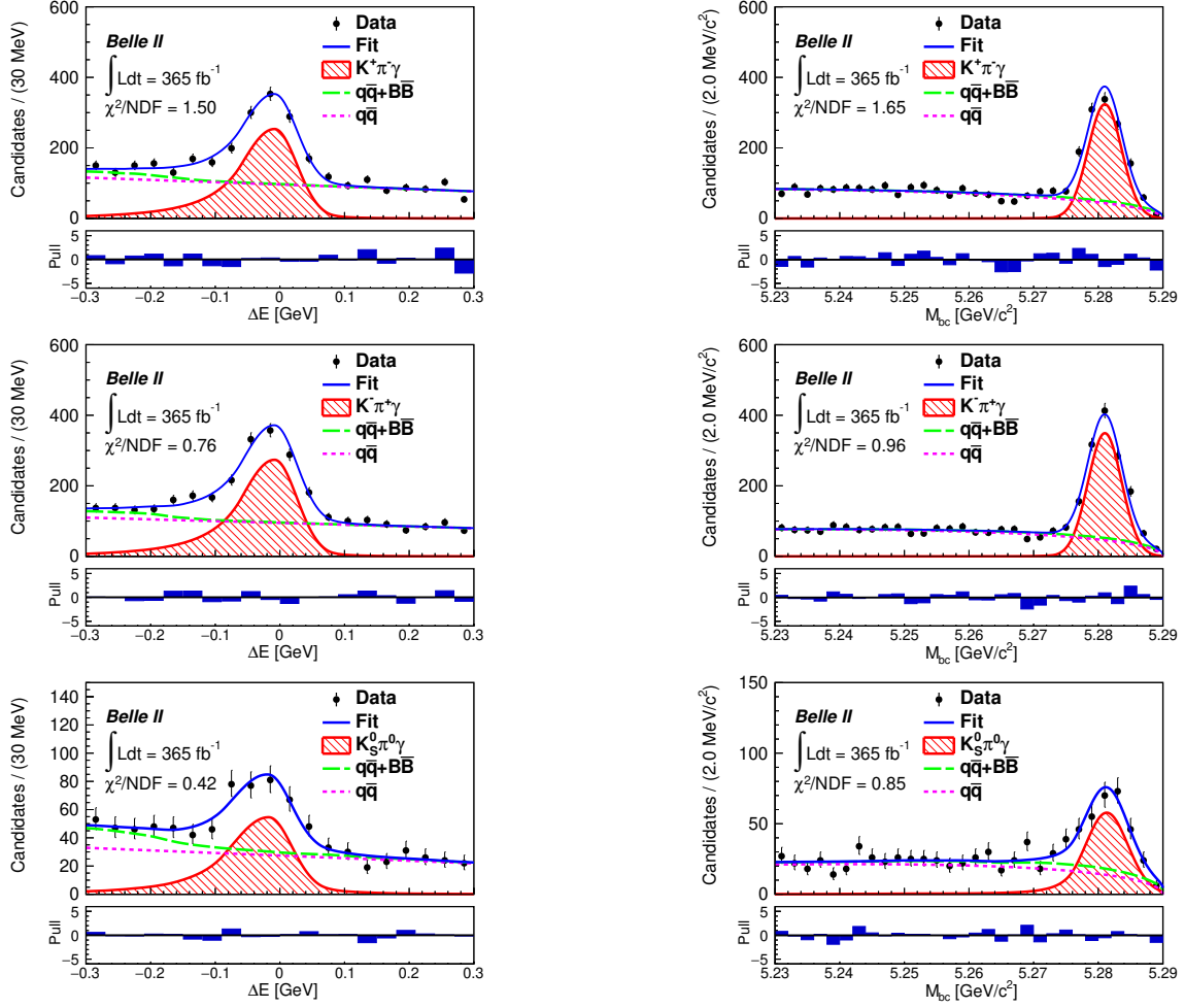
Figure 1. The \Delta E (left) and M_{bc} (right) distributions for B^0 \rightarrow K^{*0} \gamma channels with fit results superimposed. The top two rows and bottom row are for the K^\pm \pi^\mp \gamma and K_S^0 \pi^0 \gamma final state, respectively. The black dots with error bars are the data, the blue curves show the total fit, the filled red curves show the signal, the dashed green curves show the continuum background, and the dotted magenta curves show the B\bar{B} background. Lower panels show the pull, i.e., the differences between the data and fit results divided by the statistical uncertainty of the data.
