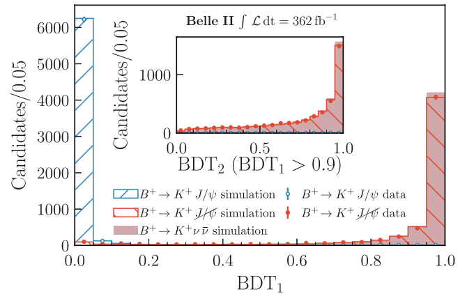
FIG. 7. Distribution of the classifier output \text{BDT}_1 (main figure) and \text{BDT}_2 for \text{BDT}_1 > 0.9 (inset). The distributions are shown before ( B^+ \rightarrow K^+ J/\psi ) and after ( B^+ \rightarrow K^+ J/\psi ) the muon removal and replacement of the kaon momentum of selected B^+ \rightarrow K^+ J/\psi events in simulation and data. As a reference, the classifier outputs directly obtained from simulated B^+ \rightarrow K^+ \nu \bar{\nu} signal events are overlaid. The simulation histograms are scaled to the total number of B^+ \rightarrow K^+ J/\psi events selected in the data.
