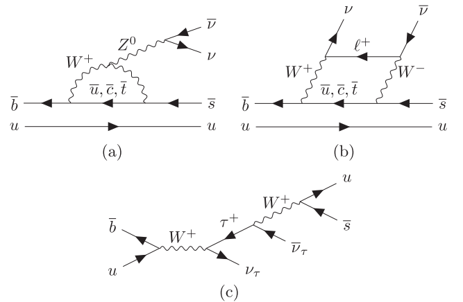
FIG. 1. Lowest-order quark-level diagrams for the B^+ \rightarrow K^+\nu\bar{\nu} decay in the SM are either of the penguin (a), or box type (b): examples are shown. The long-distance double-charged-current diagram (c) arising at tree level in the SM also contributes to the B^+ \rightarrow K^+\nu\bar{\nu} decay.
