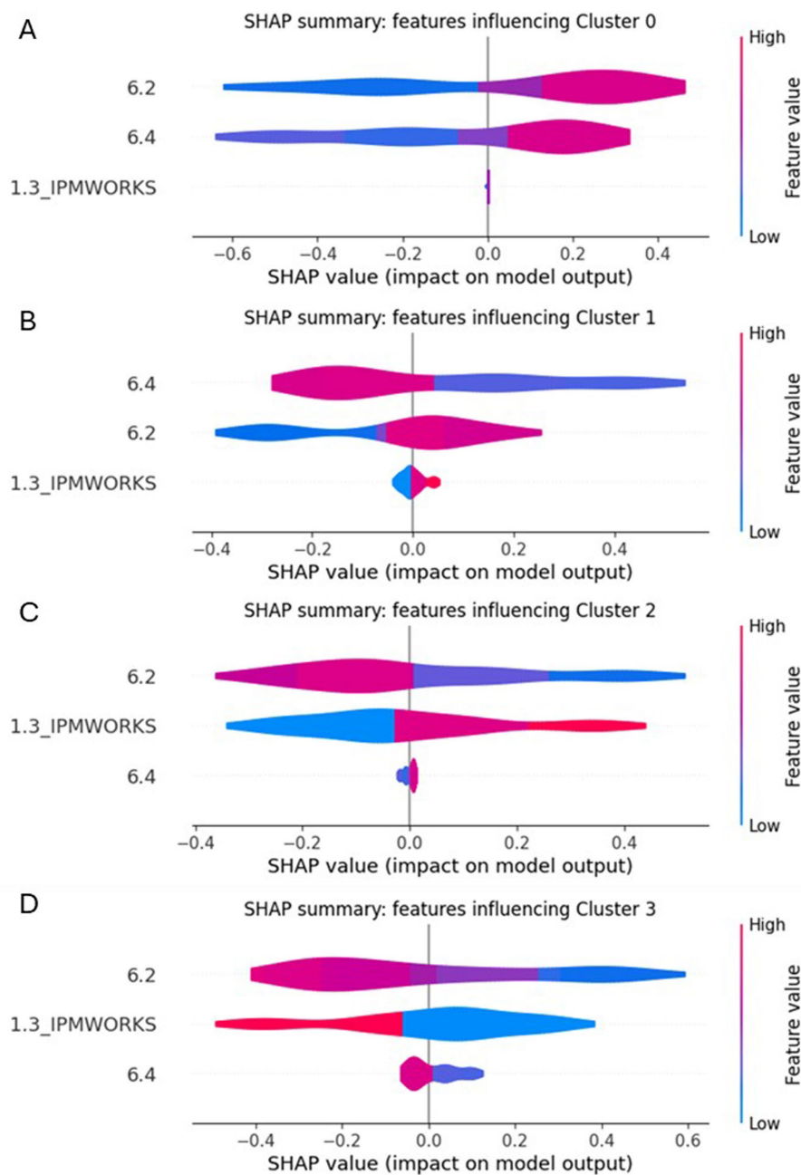
FIGURE 3 SHAP summary analysis of attributes and features determining the classification of DSS users in (A) Cluster 0; (B) Cluster 1; (C) Cluster 2; (D) Cluster 3. The attributes and features on the vertical axis in each plot are sorted in descending order of importance. The horizontal axis reports SHAP values, which quantify the impact of each feature on the likelihood of belonging to each cluster, with negative values reducing the likelihood and positive values increasing it. Red color denotes a high value, while blue color denotes a low value of the attribute or feature. Violin plots show the distribution (spread and density) of the impact of each attribute on the model's prediction. See Supplementary Table S1 for survey questions description.
