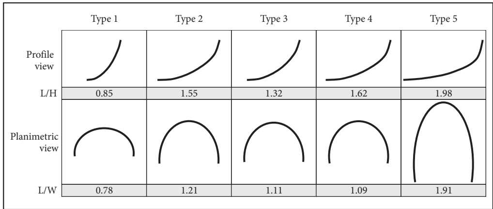
Figure 8: Schematic illustration of the five cirque types in planimetric and profile view.
