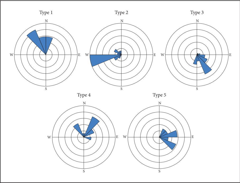
Figure 10: Percentage-based rose diagrams for median axis aspect by cirque type.
