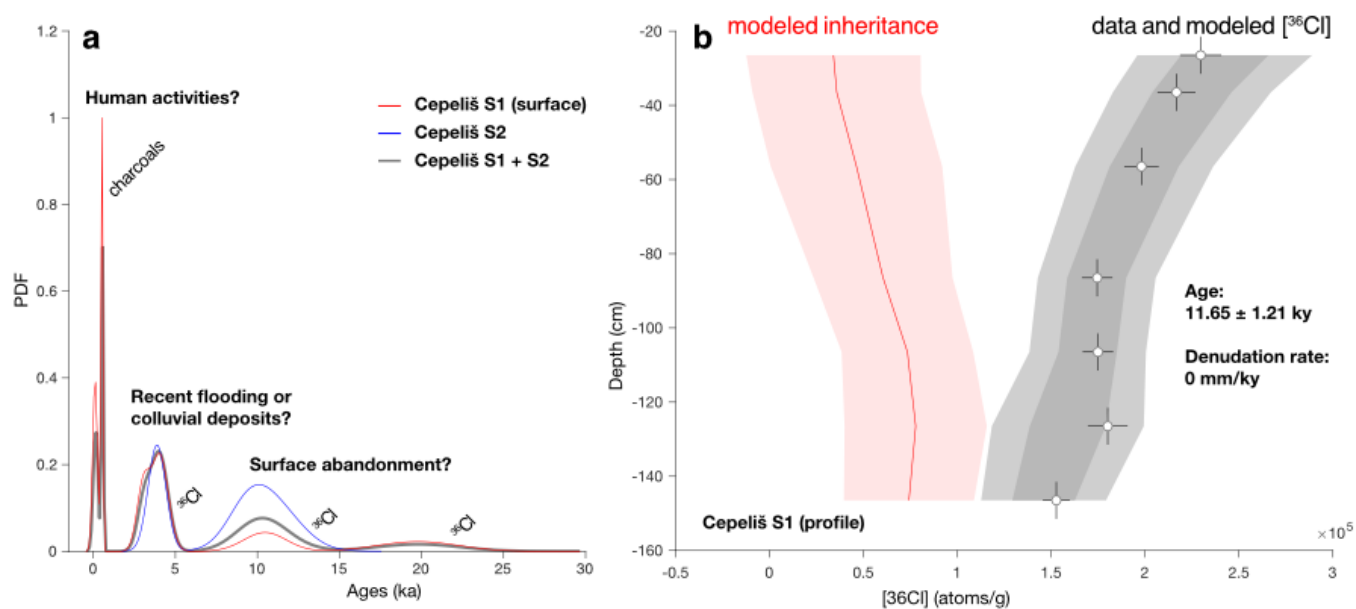
Figure 15 – Chronological constraints from Cepeliš site S1 and S2. Panel a: the probability density functions (PDF) of terrace ages considering the surface (site S1) and subsurface (site S2) ^{36}\text{Cl} CRE ages and radiocarbon ages from site S1. In red the distribution of ages from site S1, in blue from site S2 and in black the PDF with samples from both sites. Panel b: the cosmogenic depth-profile from the colluvium at the site S1 (shown in the figure 7.b). The ^{36}\text{Cl} concentrations of the data and of the best model are represented together with the estimated inheritance. These chronological data points toward a cluster of ages corresponding to the Early Holocene (9-12 ka), and another to the Late Glacial Maximum (LGM) at ~20 ka.
