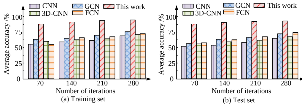
Figure 8: Average accuracy test results.
