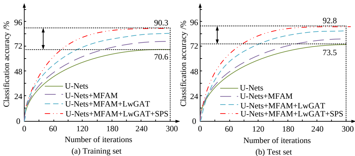
Figure 7: Ablation test.
