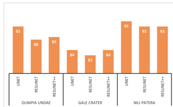
Figure 8: Accuracy assessment of results obtained from UNet, ResUNet and ResUNet++ models developed from CTX image in Olympia Undae, Gale crater and Nili Patera region
