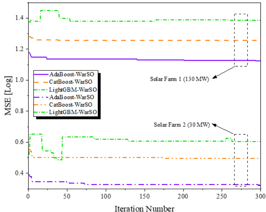
Figure 15: The convergence plots of the Cat Boost, AdaBoost, and Light GBM hybrid model
