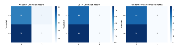
Figure 15: Confusion Matrices for XGBoost, LSTM, and Random Forest
