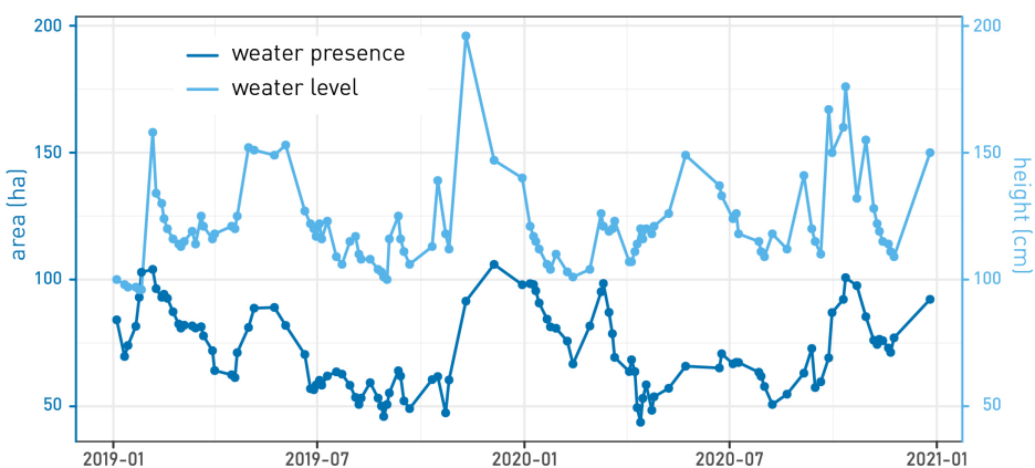
Figure 31: Time series of water presence, based on transferred endmembers, and water level measured at a gauging station in Kobariid. Data source: Slovenian Environment Agency, 2021b.
