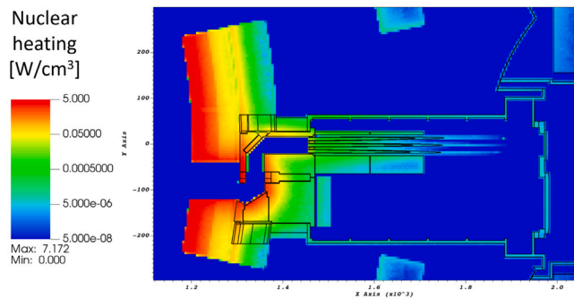
Fig. 8. Nuclear heating for case 2 in \text{W}/\text{cm}^3 , XY view through steering mirror opening ( Z = 26.8 cm).
