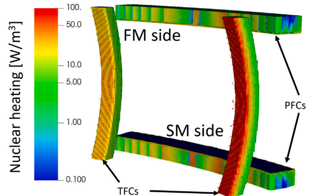
Fig. 6. Nuclear heating in superconducting magnets near EC port, i.e. Toroidal Field Coils (TFCs) and Polooidal Field Coils (PFCs), in W/m 3 for case 0.
