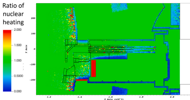
Fig. 9. Ratio of nuclear heating for the case 2 and case 0 ( \text{NH}(\text{case } 2)/\text{NH}(\text{case } 0) ), XY view through steering mirror opening ( Z = 26.8 cm). Larger red squares show locations where additional shield was added (ratio there is very large, in principle infinite as void was replaced by material) and the effect of these shields on the nuclear heating inside and outside the port is visible. Statistical uncertainties for neutron and gamma ray heating in thin components of the port are generally well below 10% but can be significantly higher in thick shields or directly behind them (as visibly by the statistical noise in those regions).
