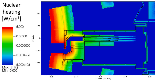
Fig. 7. Nuclear heating for case 0 in \text{W}/\text{cm}^3 , XY view through steering mirror opening ( Z = 26.8 cm).
