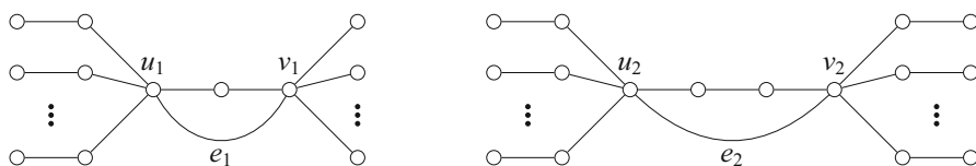
FIGURE 4. The graphs G_p (left) and G'_p (right)
