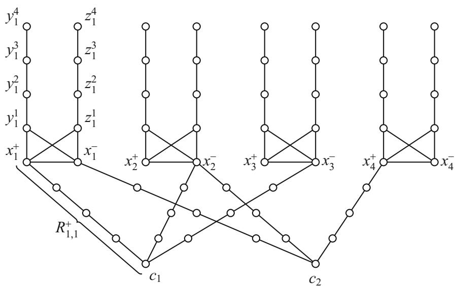
FIGURE 1. Graph G_4(F) for F = (x_1 \vee \bar{x}_2 \vee \bar{x}_3) \wedge (\bar{x}_1 \vee \bar{x}_2 \vee x_4)
