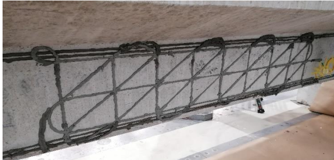
Figure 1. 2D sensor arrangement for shear monitoring
