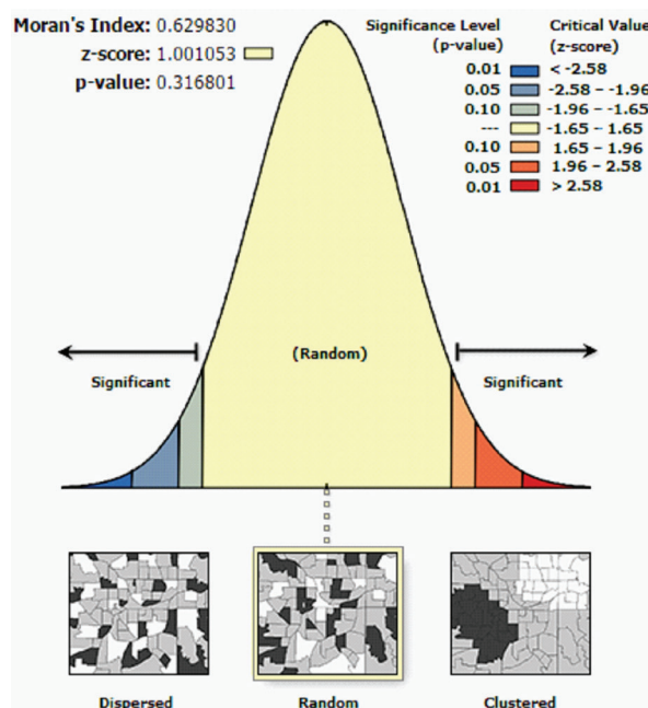
Figure 3: Output of Global Moran's I.
