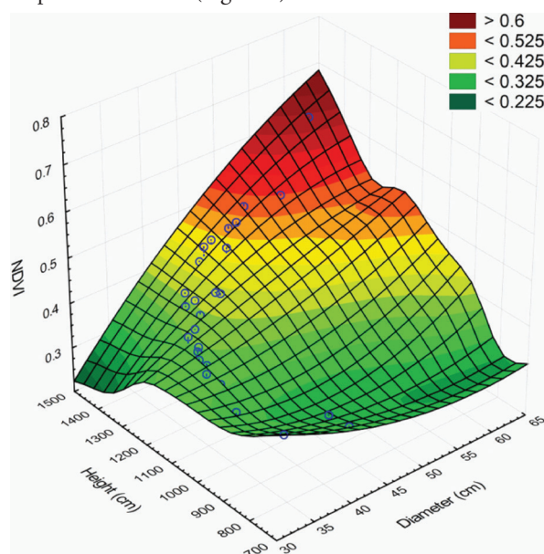
Figure 5: 3D surface plot of NDVI against height and DBH.
