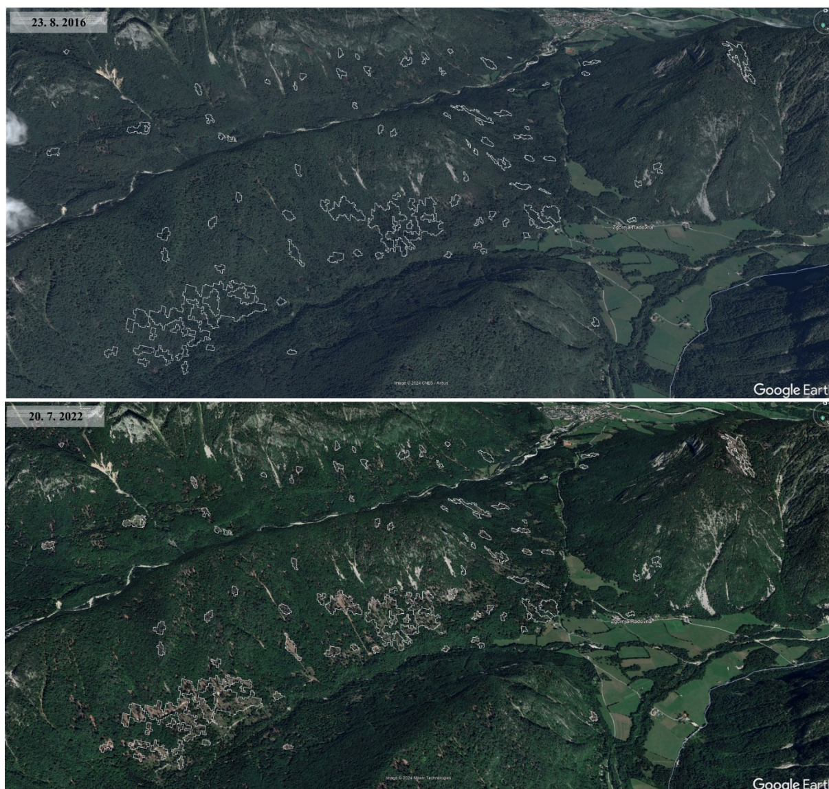
Appendix 1: An extract from the final data set of the bark beetle mask. The first image represents the situation in 2016, while the second image shows the bark beetle area with white polygons. The background is © Google Earth History Aerial photos.
