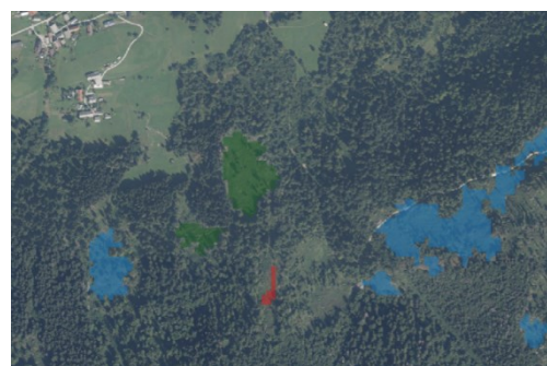
Figure 6. Prepared geospatial dataset of bark beetle detection in different years. Red area is affected in 2018, blue in 2019 and green in 2021.
