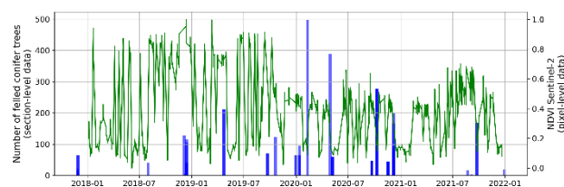
Figure 3. Temporal relationship between the number of felled conifers (blue bars, derived from the TIMBER database at forest compartment level) and Sentinel-2 NDVI values (green line, pixel-level data) at a bark beetle-infested site in the Pokljuka region. The NDVI time series shows a decrease in vegetation greenness coincides with the increase in remediation activities, indicating a correspondence between remotely sensed changes and ground-based observations.
