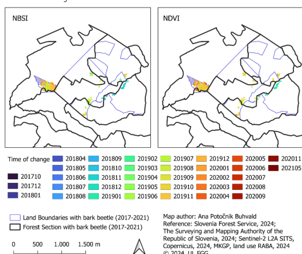
Figure 4. Time of detected spectral change based on CuSum analysis of NBSI (left) and NDVI (right) time series. Colours represent the estimated month and year of change between 2017 and 2021. Black outlines indicate forest sections with bark beetle-
