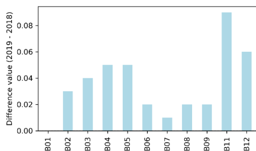
Figure 7. Yearly difference values (2019–2018) for all Sentinel-2 bands (B01–B12). The analysis highlights the most significant spectral bands for detecting bark beetle-induced changes, with SWIR bands (B11, B12), the red band (B04), and the red-edge band (B05) showing the largest differences. These features indicate key spectral responses to vegetation stress and disturbance during the infestation period.
