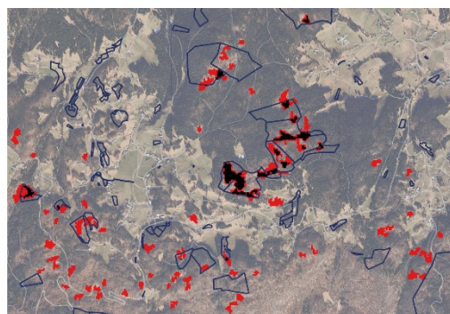
Figure 5. Final bark beetle disturbance mask (black), change detection mask from Sentinel-2 (red), and forest compartments with insect-related logging from the TIMBER database (blue) overlaid on aerial imagery.
