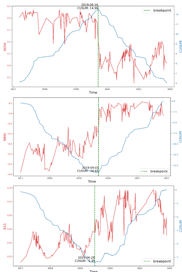
Figure 2. Example of CUSUM-based change detection using NDVI (top), NBSI (centre), and SWIR band B11 time series (bottom) at a coniferous forest site in Pokljuka. The vertical line indicates the point of detected change corresponding to the probable time of disturbance.
