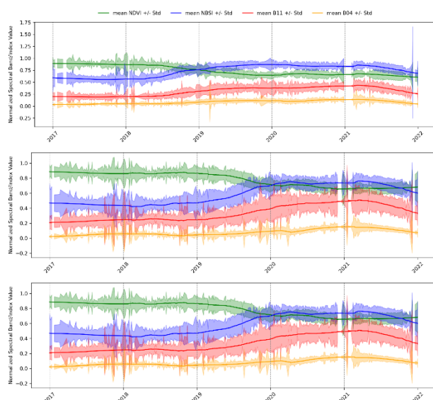
Figure 8. Time series of normalized spectral band/index values for NDVI (green), NBSI (blue), B11 (red), and B04 (orange) with mean values and standard deviation ( \pm std) for 2018 (first), 2019 (second) and 2020 (third) which shows notable changes during the bark beetle infestation period for specific year and dataset.
