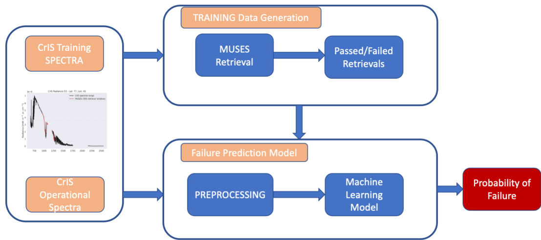
Figure 2. Flow chart describing the ML pipeline for the failure prediction model.
