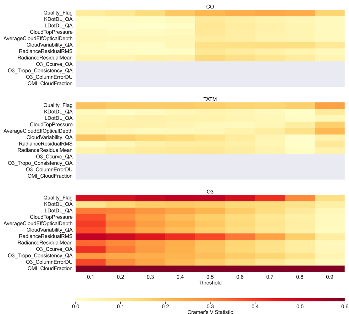
Figure 13. Cramér's V statistics for the AIRS-OMI dataset between quality flags and the independent predicted dataset for varying thresholds of pass or failure, ranging from 0.1 to 0.9, for the three gases: CO, TATM, and O 3 . A small association is defined by values of 0.1–0.3, a medium association is defined by values of 0.3–0.5, and a large association is defined by values of > 0.5 .
