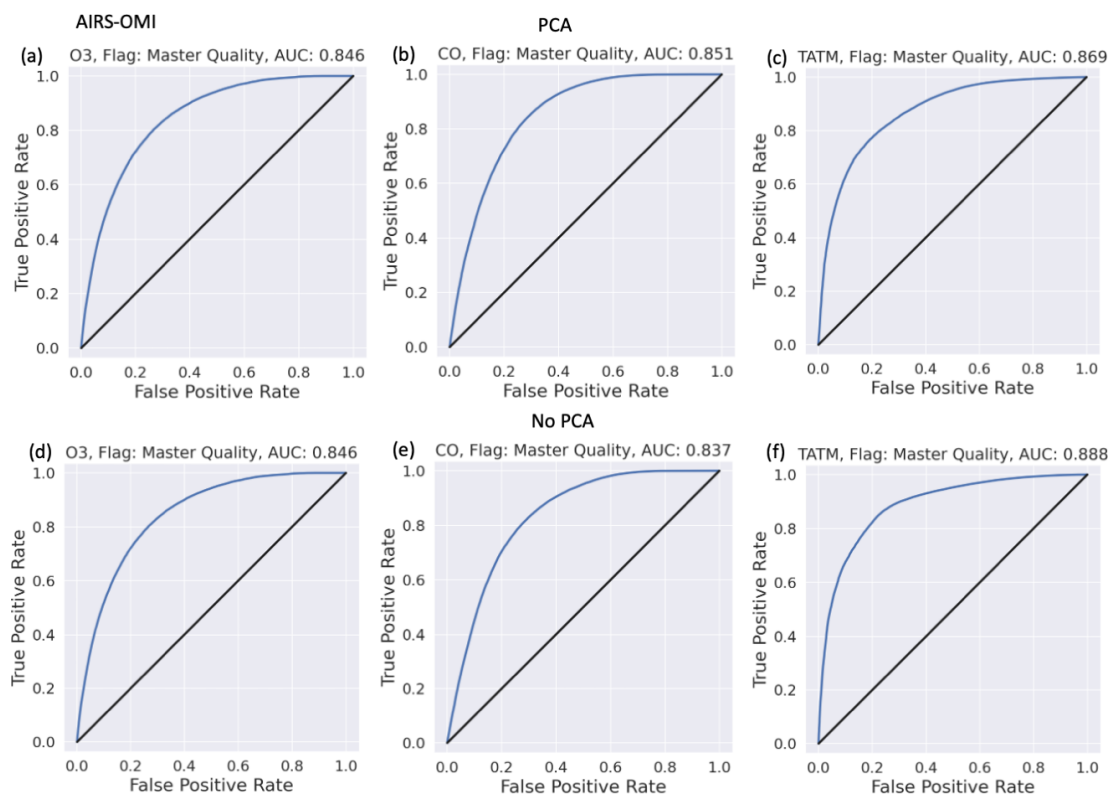
Figure 7. ROC curves for training scenarios 7–8; all figure aspects are as in Fig. 5 but showing AIRS-OMI ML results for both the PCA and non-PCA cases.
