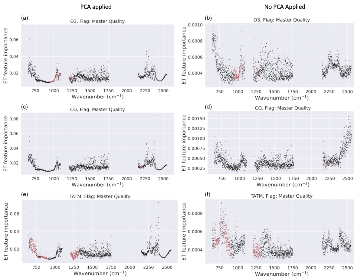
Figure 8. Feature importance of the CrIS full-band models. Panels (a), (c), and (e) show results for the models including PCA (top to bottom: ozone, CO, and TATM). Panels (b), (d), and (f) show the results for the models without PCA, with the same target ordering in rows. The red dots indicate the spectral windows of the retrievals depending on the trace gas, and the black dots indicate wavelengths outside of the spectral windows.
