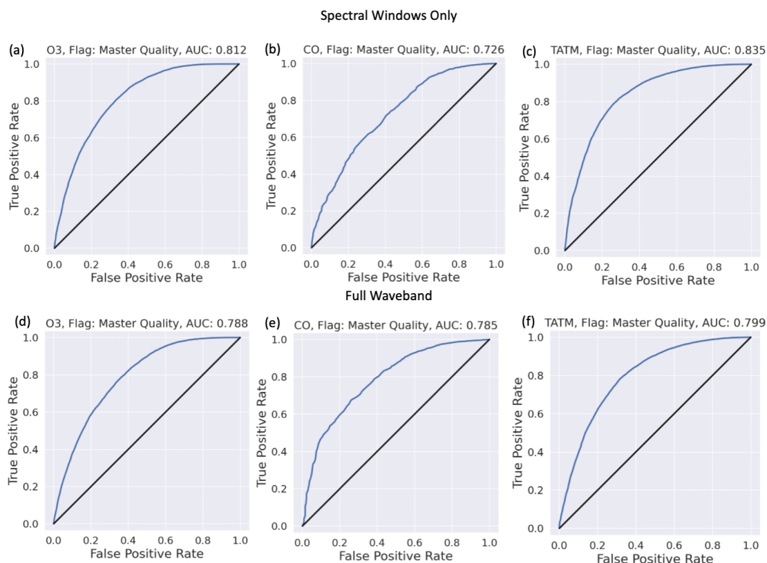
Figure 5. ROC curves for training scenarios 1–6, with the target quantities of ozone, carbon monoxide, and TATM (from left to right) from CrIS input into the ML model having been passed through a PCA. Panels (a)–(c) show ROC curves when the ML tool is trained only on the spectral windows identified in Tables A1, A3, and A4. Panels (d)–(f) present ROC curves for when the ML tool is trained on the full CrIS spectral range. The blue lines represent the ROC curve for a specific model, while the black 1 : 1 line represents an uninformed classifier model. The title for each panel indicates the target trace gas, as well as the AUC score for the target and/or window case.
