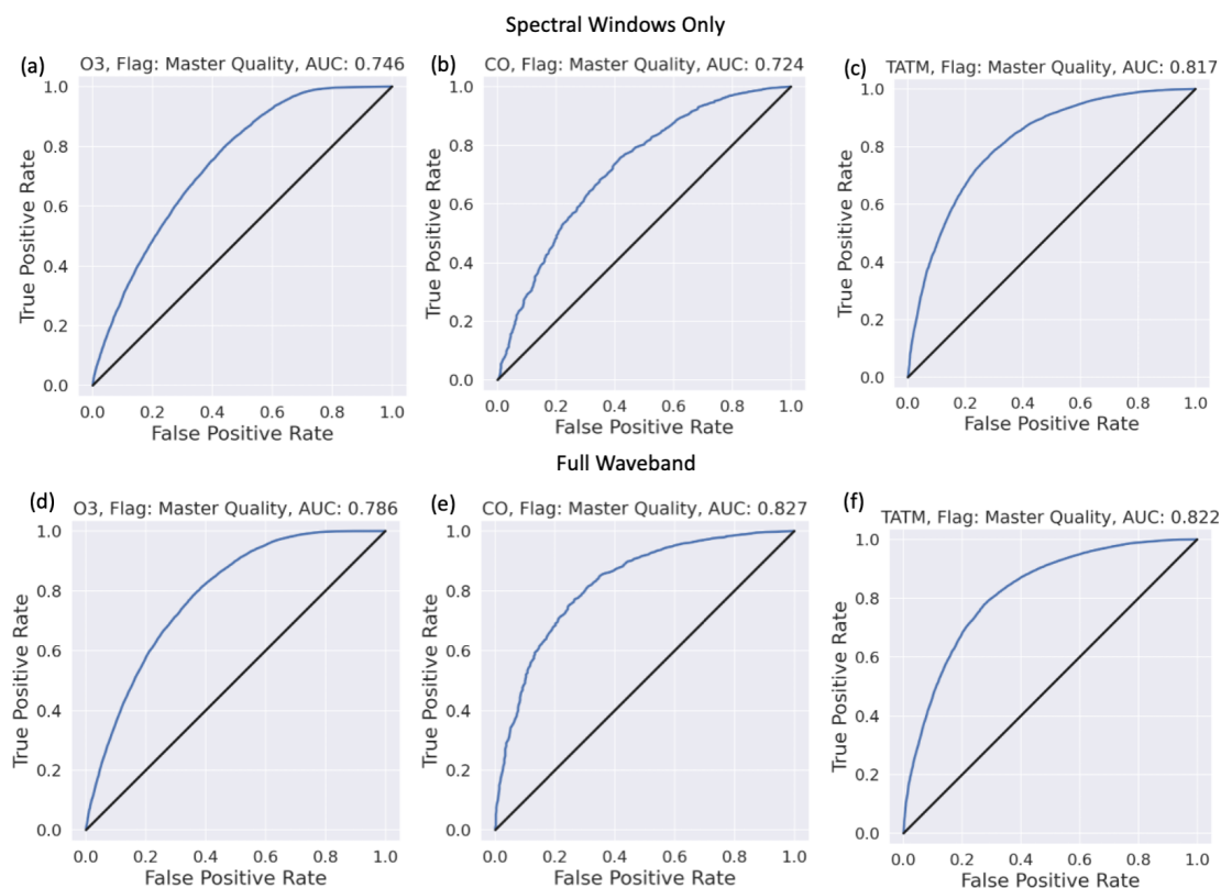
Figure 6. As in Fig. 5 but showing results for the ML model without PCA.
