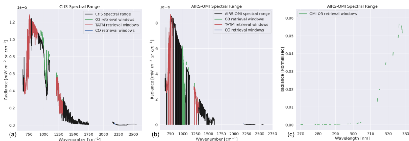
Figure 1. Example spectral windows. Panel (a) shows windows for ozone, CO, and TATM with respect to CrIS radiance. Panel (b) shows the same as the left-hand panel but for AIRS radiance. Panel (c) shows the ozone spectral windows in the OMI radiance as a part of the AIRS-OMI retrieval.
