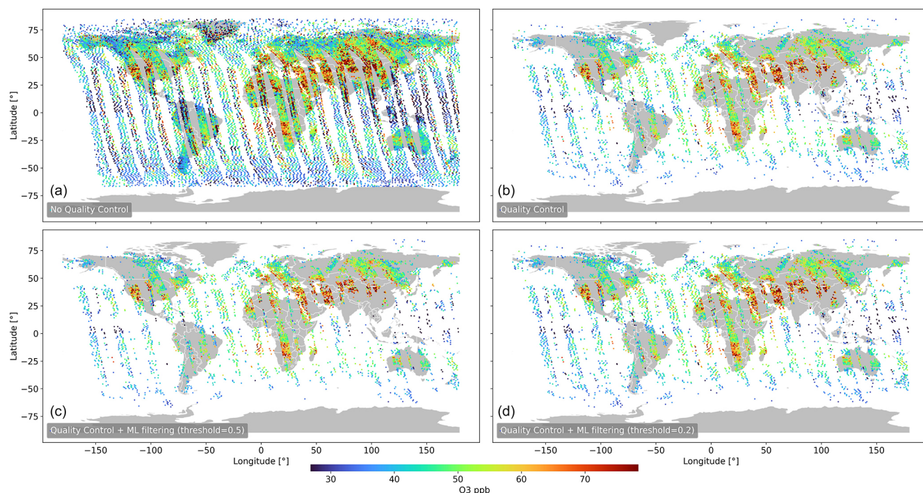
Figure 15. Impact of applying the ML filter to MUSES ozone retrievals for AIRS-OMI. Daytime retrievals at 681 hPa pressure level using the standard MUSES processing with no quality-controlling (a) and with standard quality-controlling flags applied (b). The ML filter is applied with thresholds of 0.5 (c) and 0.2 (d), with the remaining data having been quality-controlled.
