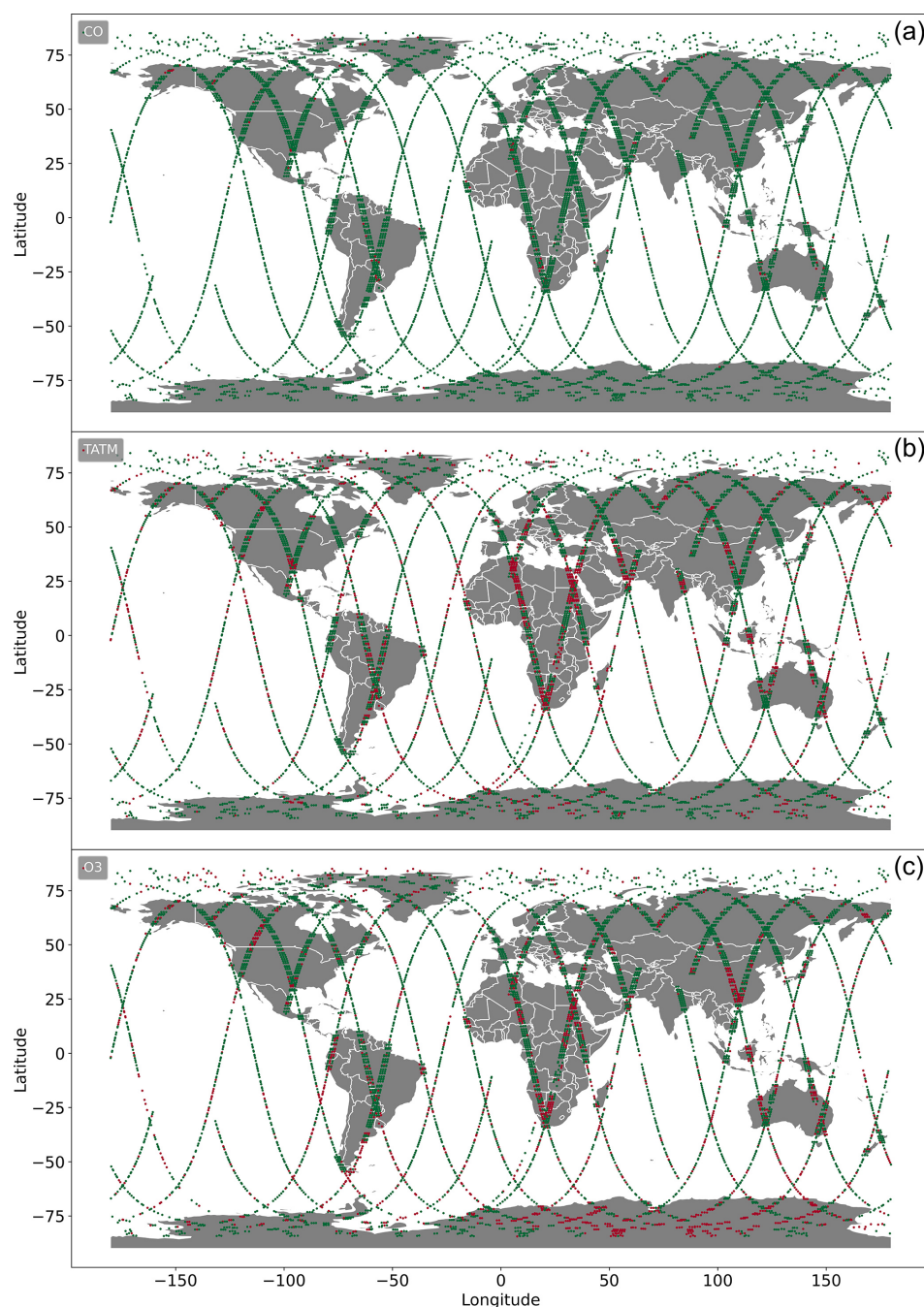
Figure 4. Global distributions of failed retrievals on 15 January 2020 for MUSES CrIS carbon monoxide (a), temperature (b), and ozone (c) profile retrievals. Green markers indicate passed retrievals, and red markers show failed retrievals.
