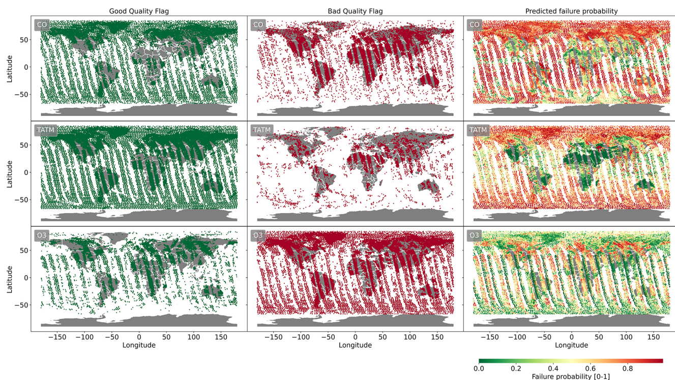
Figure 11. As in Fig. 10 but for AIRS-OMI retrievals.
