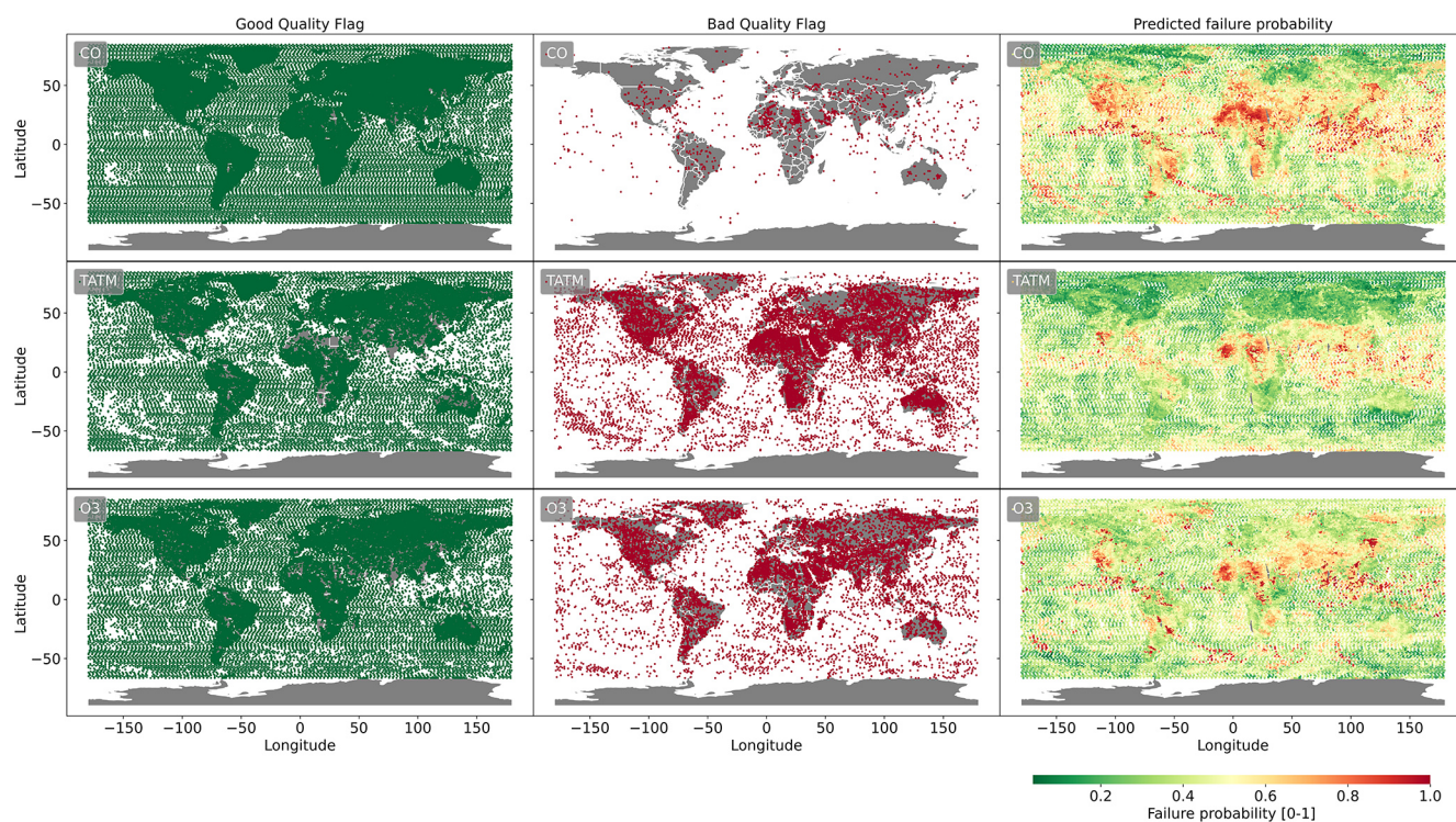
Figure 10. Quality flags from MUSES CrIS retrievals of CO, TATM, and O 3 on 12 August 2020, where the left-hand column (green) indicates triggering of the good-quality flag, and the middle column (red) indicates the triggering of bad-quality flags. Predicted probability of failure [0–1] from ML models for CO, TATM, and O 3 (the rows) on the same day can be seen in the right-hand column
