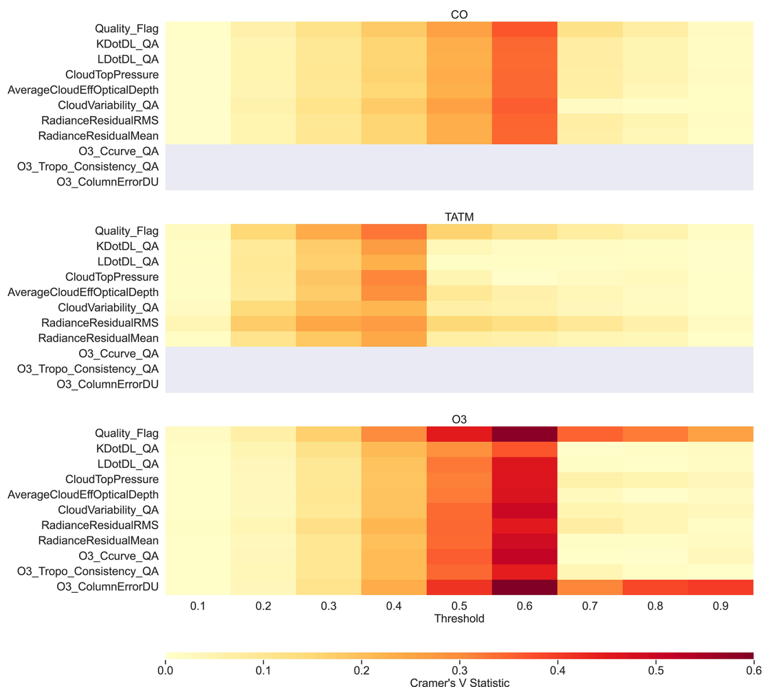
Figure 12. Cramér's V statistics for the CrIS dataset between quality flags and the independent predicted dataset for varying thresholds of pass of failure, ranging from 0.1 to 0.9, for the three gases: CO, TATM, and O 3 . A small association is defined by values of 0.1–0.3, a medium association is defined by values of 0.3–0.5, and a large association is defined by values of > 0.5 .
