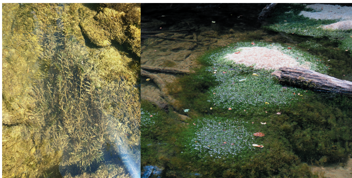
Slika 9: Obarjanje kalcijevega karbonata pri kodravem dristavcu ( Potamogeton crispus ; levo) in parožnici ( Chara sp.; desno). Figure 9: Calcium carbonate precipitation on curly-leaved pondweed ( Potamogeton crispus ; left) and stonewort ( Chara sp.; right).
