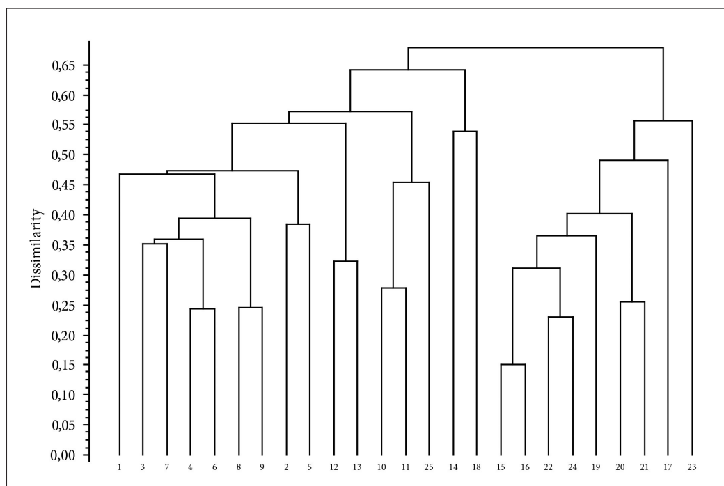
Figure 3: Dendrogram of stands at springs in the subalpine and alpine belt of the Julian Alps (UPGMA, 1-similarity ratio). Slika 3: Dendrogram sestojev ob izvrih v subalpinskem in alpskem pasu Julijskih Alp (UPGMA, 1-similarity ratio).
