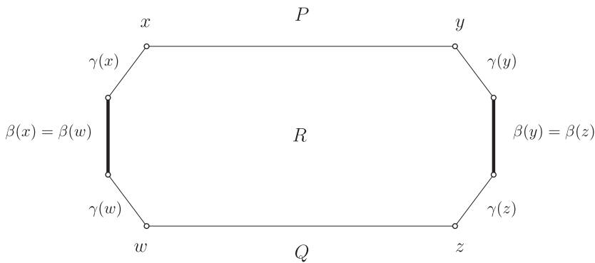
Figure 2: A cage for the robber encloses robber's territory R . Each cage is bounded by two "internally geodesic" paths P and Q (geodesic inside \overline{R} ), four short geodesics \gamma(u) , with \ell(\gamma(u)) \leq \varepsilon/2 , u \in \{x, y, w, z\} , and two boundary segments \beta(x) = \beta(w) and \beta(y) = \beta(z) (shown as bold lines). Each of the constituents can be a single point. Moreover, \beta(x) (and \beta(y) ) can be empty, in which case \gamma(x) = \gamma(w) ( \gamma(y) = \gamma(z) , respectively). Each of the points depicted as a small circle is either a vertex in \mathcal{T}_0 or a point on an edge in \mathcal{T}_1 . The paths P , Q , and \gamma(u) need not be contained in the 1-skeleton of \mathcal{T} .
