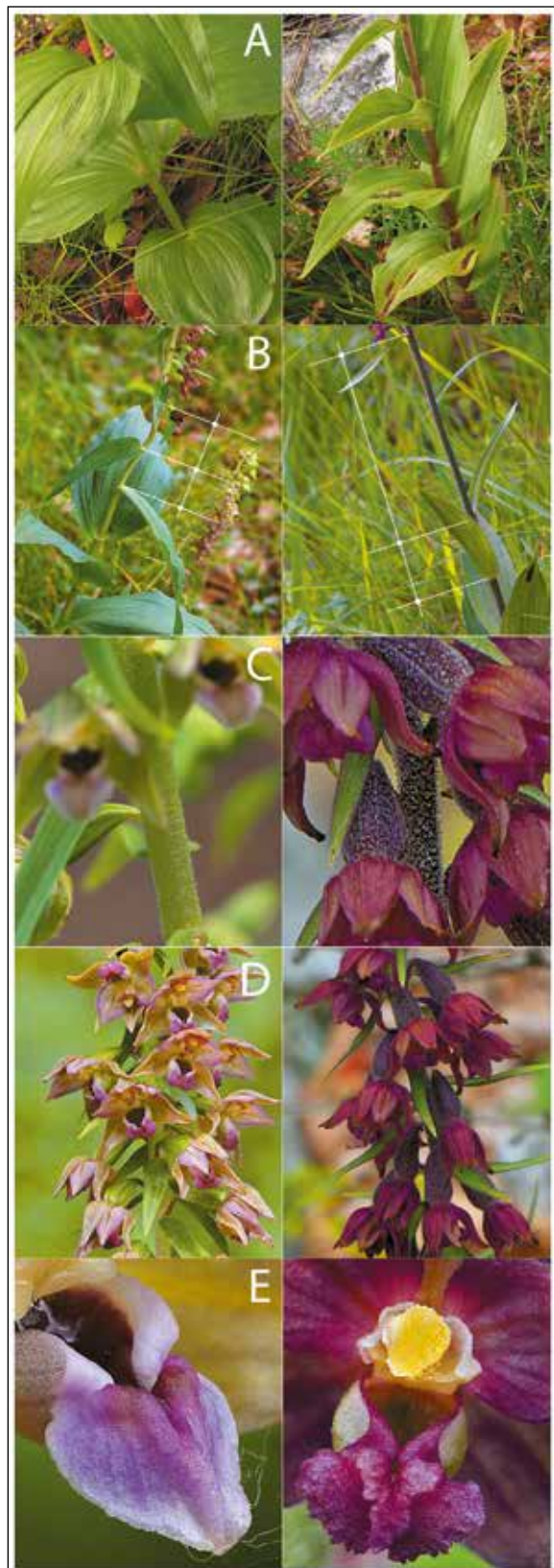
Figure 2: The typical traits of parental plants (left Epipactis helleborine , right Epipactis atrorubens ) considered in assessing the degree of hybridity (DH). A: shape and arrangement of lower leaves (LVSH, LVAR); B: the ratio of the length of the last to the length of the last but one internode (INTR); C: pubescence and color of the inflorescence axis (STPB, STCO); D: flower color (FLCO); E: surface structure of protuberances at the base of epichile and their transition to the epichile surface (ECON). Photo: A. Trnkoczy.
