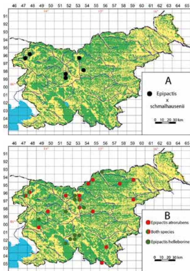
Figure 1: Visual representation of the localities of the studied taxa from the FloVegSi database. A: MTB quadrants with Epipactis × schmalhauseni ; B: MTB quadrants with the parental plants.
