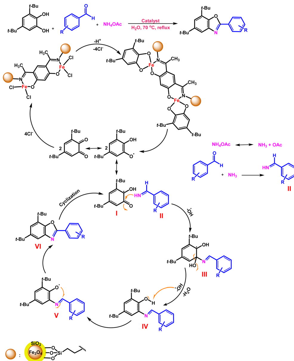
Scheme 5 Proposed mechanism for benzoxazoles synthesis reaction of the \text{Fe}_3\text{O}_4@(\text{SiO}_2\text{-APTES})\text{-Fe}_2\text{L}^{\text{DAR}} catalyst.
