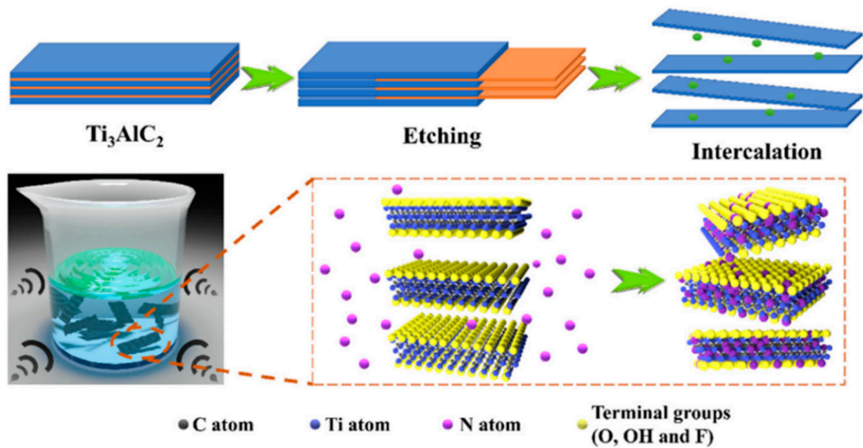
Figure 2. Stepwise procedure for ultrasound-assisted synthesis of N-doped MXene. (Reprinted from [29] with copyright permission for figure obtained from Elsevier).
