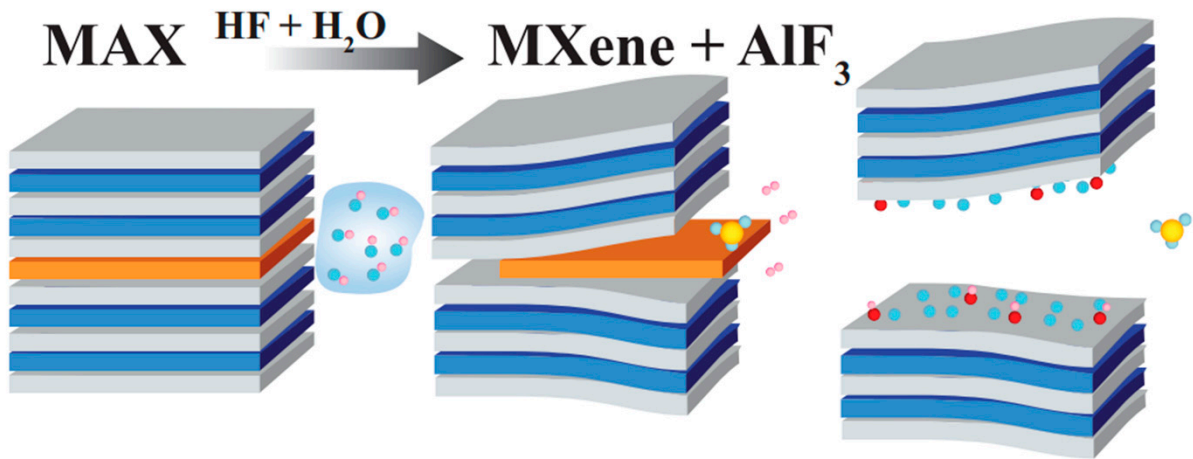
Figure 4. Exfoliation of \text{Ti}_3\text{AlC}_2 MAX phase using HF/ \text{H}_2\text{O} . (Reprinted with permission from [38] Copyright (2016) American Chemical Society).
