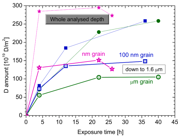
Fig. 4. D amounts as a function of exposure time for the different-grained samples exposed to 300 eV D ions at 450 K, as obtained from the D depth profiles shown in Fig. 2. The D amounts down to 1.6 \mu\text{m} (empty symbols) and D amounts within the whole analysed depth (full symbols) are shown.
