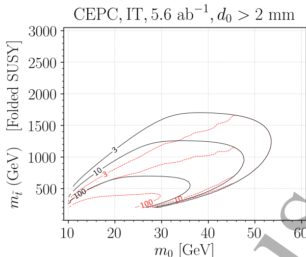
FIG. 40: Sensitivity reaches of \log_{10}(N_{\text{signal}}) at the CEPC for the Folded SUSY model.
