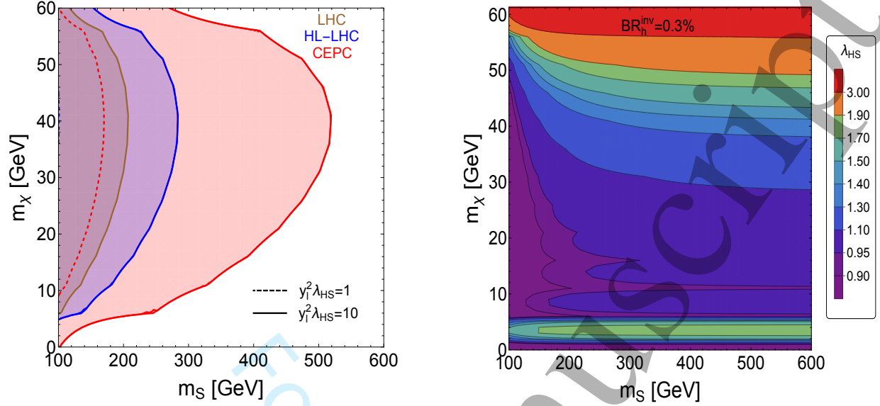
FIG. 12: Left: The Higgs portal coupling \lambda_{HS} (Eq. 3) and the fermion portal coupling y_\ell (Eq. 2) can induce the Higgs invisible decay h \rightarrow \bar{\chi}\chi at one-loop level. Constraints on the coupling combination y_\ell^2 \lambda_{HS} are derived from searches for invisible Higgs decays at the LHC, HL-LHC ( BR_{h \rightarrow inv} < 3.5\% ), and CEPC ( BR_{h \rightarrow inv} < 0.3\% ). The recent CEPC Technical Design Report (TDR) [14] projects an improved limit of BR_{h \rightarrow inv} < 0.07\% with an upgraded integrated luminosity of 20 \text{ ab}^{-1} during Higgs operation, which could further tighten the bound on y_\ell^2 \lambda_{HS} by a factor of two. Right: For each mass point (m_S, m_\chi) , the fermion portal coupling y_\ell is set to its thermal value y_\ell^{th} , as required by the observed dark matter relic abundance. Constraints on the Higgs portal coupling \lambda_{HS} are then derived using the CEPC limit on the invisible Higgs branching fraction Br(h \rightarrow inv) < 0.3\% .
