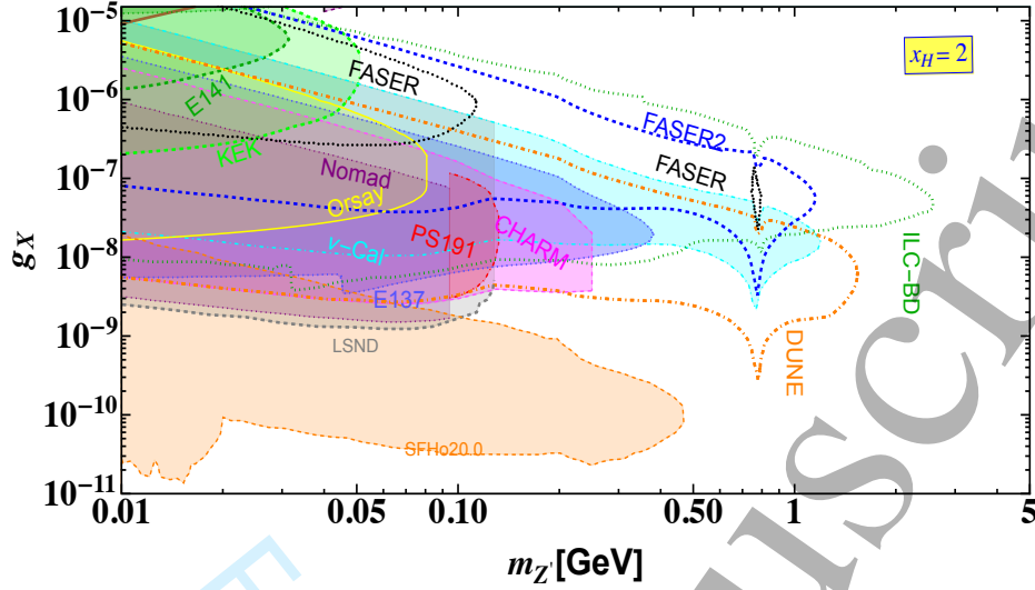
FIG. 58: Limits in the m_{Z'} – g_X plane for x_H > 0 and x_\Phi = 1 considering 10 MeV \leq m_{Z'} \leq 5 GeV, showing the regions that could be probed by FASER, FASER2, ILC-Beam dump, and DUNE. The parameter space is compared with existing bounds from different beam-dump experiments and a cosmological observation of supernova SN1987A (SFHo20.0), respectively. Taken from Ref. [432].
