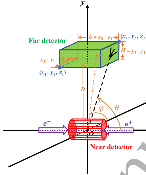
FIG. 48: The sketch displays the main detector (near detector, abbreviated as ND) and an example far detector. The dashed line indicates that one LLP is produced at the IP, travels through the main detector and decay inside the far detector. Taken from Ref. [76].
