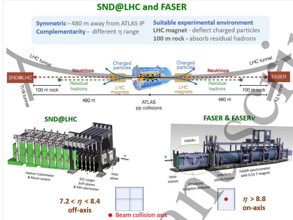
FIG. 46: Schematic pictures of the SND@LHC, FASER \nu , and FASER experiments. Taken from Ref. [400].
