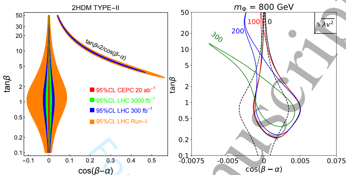
FIG. 98: The allowed region in the plane of \cos(\beta - \alpha) - \tan\beta at 95% C.L. for the Type-II of 2HDM, given LHC and CEPC Higgs precision measurements at tree level (left) and loop level under CEPC (right). For the tree-level global fit, the special “arm” regions for the Type-II is the wrong-sign Yukawa region. The right panel shows the parameter space varying the value \sqrt{\lambda v^2} with m_A = m_H = m_{H^\pm} = m_\Phi = 800 \text{ GeV} . The tree-level only global fit results are shown by the dashed black lines for comparison. More details are shown in Ref. [598].
