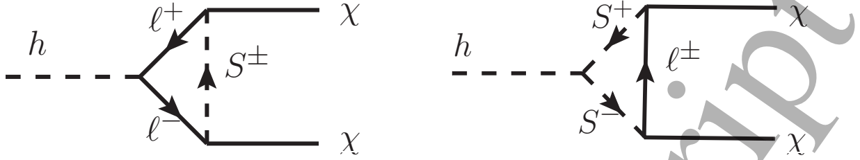
FIG. 11: The one-loop induced Higgs invisible decay (from Ref.[46]). The cross-diagrams for Majorana fermion \chi are not shown here but are included in the calculation.
