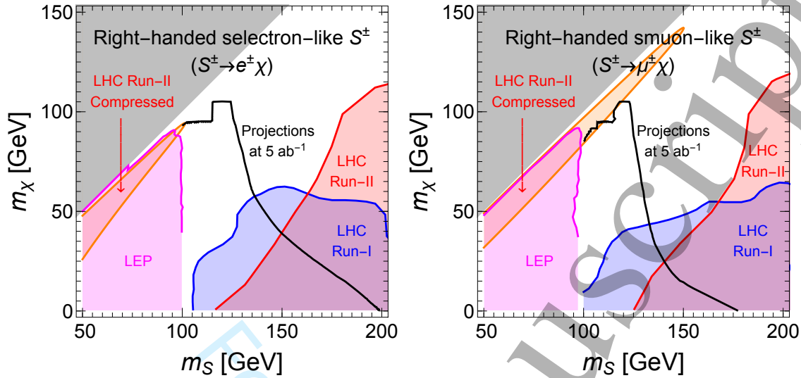
FIG. 24: Current constraints on right-handed selectron-like ( Left Panel ) and smuon-like ( Right Panel ) scalar S in the (m_{\text{DM}}, m_S) plane [46]. Black lines show CEPC projections at 5 \text{ ab}^{-1} from the Drell-Yan process e^+e^- \rightarrow S^{\pm(*)}S^\mp with S^\mp \rightarrow \ell^\mp \chi (allowing one off-shell S^{\pm(*)} ). Sensitivity extends to m_S > \sqrt{s}/2 = 120 \text{ GeV} via off-shell S^{\pm(*)} contributions. The CEPC 360 GeV operation could further extend the constraints, complementing the coverage to LEP and LHC exclusions.
