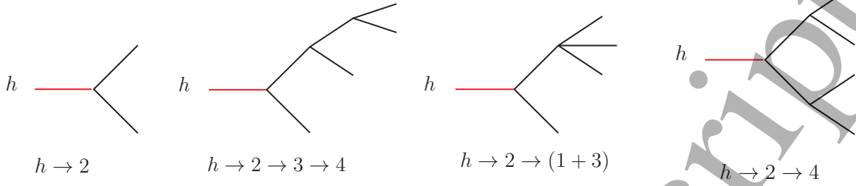
FIG. 6: Representative topologies of the Higgs exotic decays [34].
