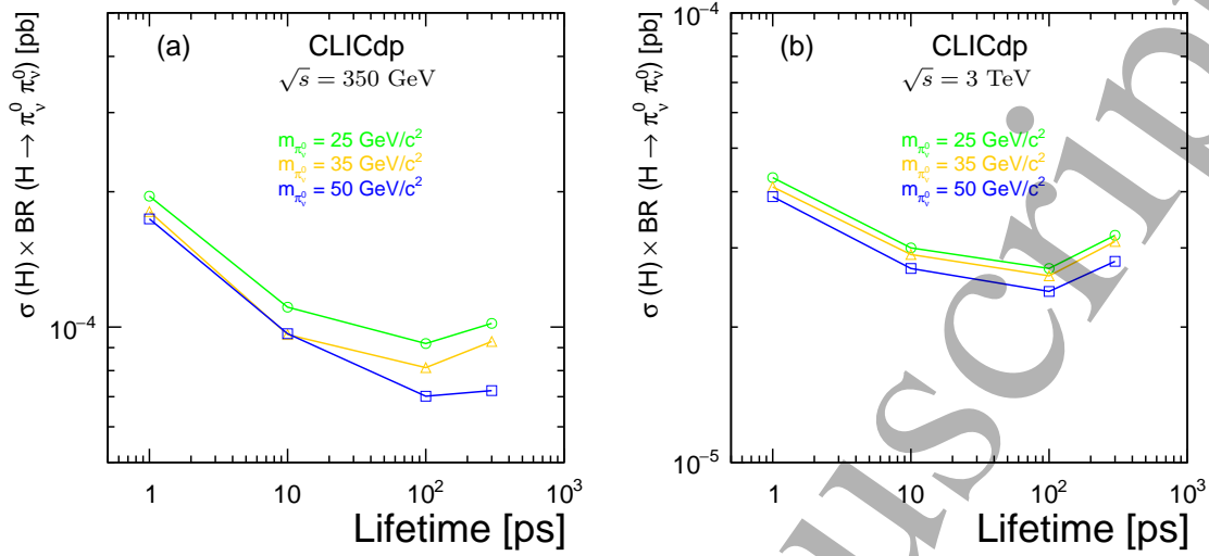
FIG. 42: Expected 95% CL cross-section upper limits on the \sigma(H) \times BR(H \rightarrow \pi_v^0 \pi_v^0) , within the model [388], for three different \pi_v^0 masses: 25 GeV (green), 35 GeV (yellow), 50 GeV (blue), as a function of \pi_v^0 lifetime for \sqrt{s} = 350 GeV (a) and \sqrt{s} = 3 TeV (b).
