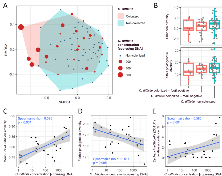
Fig. 1 C. difficile associated gut microbial community characteristics. (A) C. difficile colonization associated characteristics presented with non-metric multidimensional scaling (NMDS) plot illustrating beta diversity using Bray-Curtis dissimilarities, with colours indicating C. difficile colonization status and dot size representing C. difficile concentration. (B) Alpha diversity analysis depicted by Shannon diversity and Faith's phylogenetic diversity. (C, D and E) C. difficile concentration (ddPCR; copies per ng DNA) associated changes in (C) mean Bray-Curtis dissimilarity, (D) Faith's phylogenetic diversity and (E) Escherichia/Shigella (ZOTU1) relative abundance. All correlations are supported with Spearman's rho and significance
