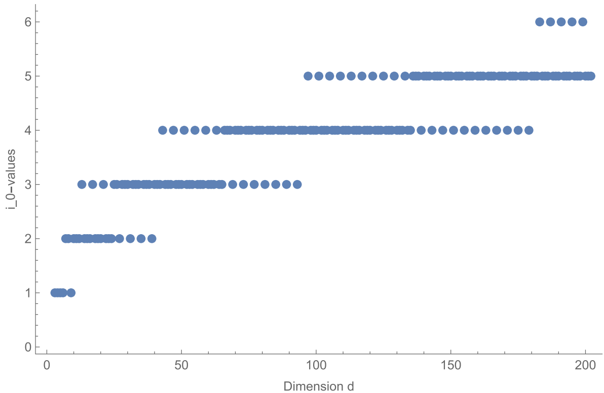
Fig. 2. Points represent the pairs (d, i_0) such that a d -box B = \left[ \frac{i_0}{i_0+1}, 1 \right]^d , obtained by Theorem 2 , is a maximal positive volume V_Q(B) box in dimension d over all d -quasi-copulas and over all d -boxes.
