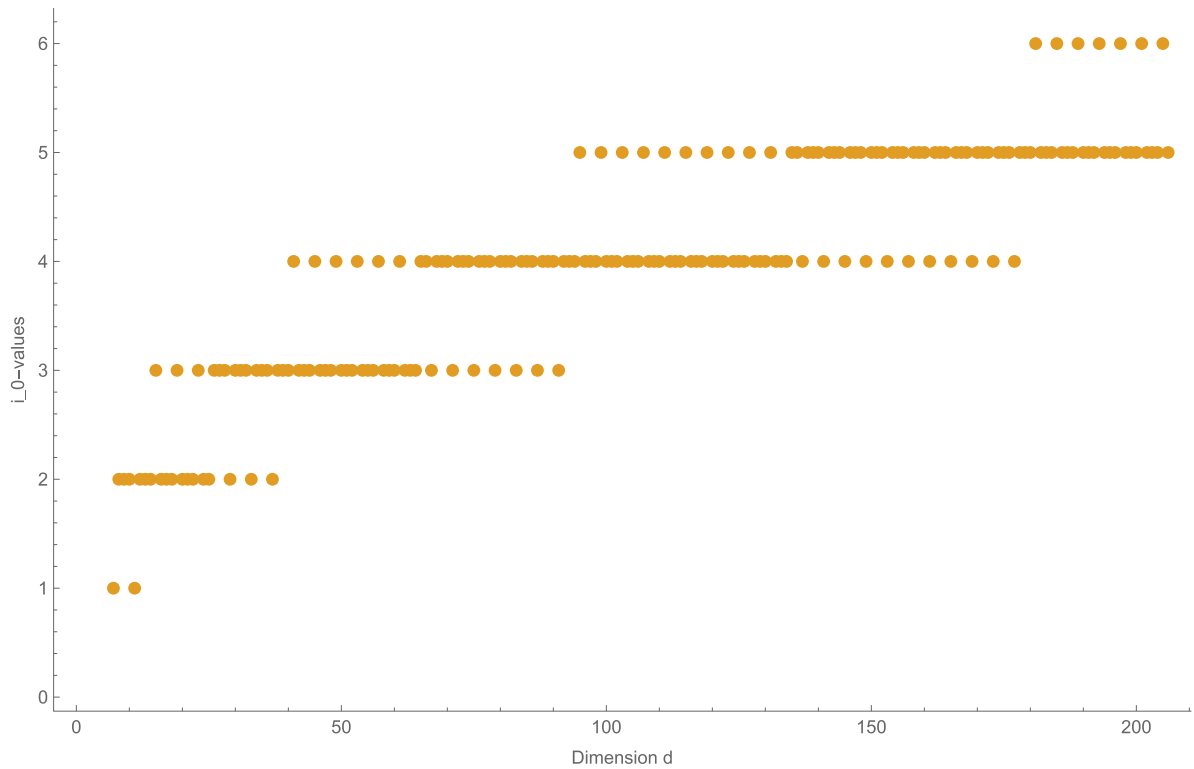
Fig. 1. Points represent the pairs (d, i_0) such that a d -box B = \left[ \frac{i_0}{i_0+1}, 1 \right]^d , obtained by Theorem 1 , is a maximal negative volume V_O(B) box in dimension d over all d -quasi-copulas and over all d -boxes.
