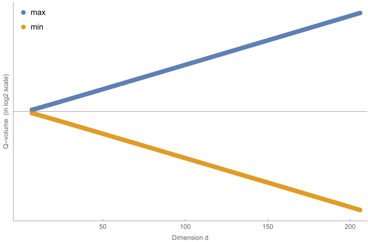
Fig. 4. Blue (and orange) points represent the volumes of boxes with maximal (and minimal) volume over all d -quasi-copulas and over all d -boxes. The x -axis represents the dimension d , while the y -axis represents the value of the volume in the logarithmic scale with base 2.
