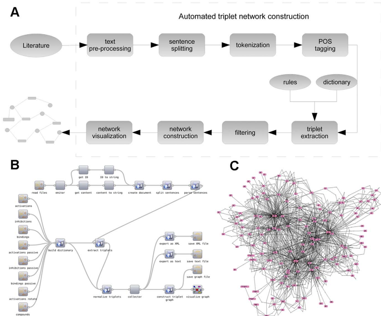
Figure 5. Overview of the Bio3graph methodology, its implementation and a sample output. A) Schematic representation of the Bio3graph methodology. Text processing is performed in a workflow according to the boxes in the schematic diagram resulting in a network of ( component1, reaction, component2 ) triplets. B) Bio3graph as a workflow implemented in Orange4WS. C) The triplet network extracted and composed by Bio3graph. The output network (consisting of 129 components and 1,132 reactions) is visualised with the Biomine visualizer and made available in Supporting Information S5. doi:10.1371/journal.pone.0051822.g005
