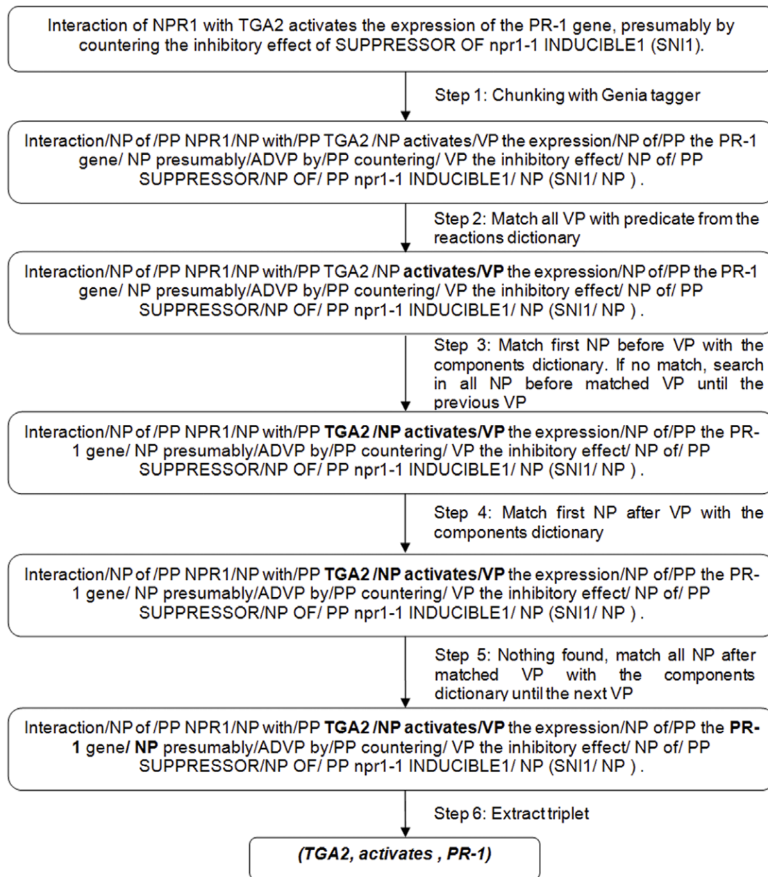
Figure 9. Illustration of the triplet extraction. We show a part of the flow from input of POS tagging box from Figure 5 until output of triplet extraction box of the same figure. The input to the Genia POS tagger is previously pre-processed sentence. After the shallow parsing with Genia POS tagger, the algorithm performs the step 2. The final output from the triplet extraction part of Bio3graph approach is a triplet in the form ( subject, predicate, object ) which will be then transformed and visualised as an edge-labelled graph with the Biominer visualiser. doi:10.1371/journal.pone.0051822.g009
