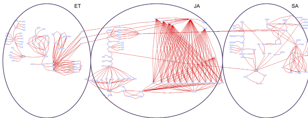
Figure 3. Manually constructed PDS model topology visualised as an edge-labelled graph. This graph, consisting of 175 nodes and 387 edges, is provided in Supporting Information S2 as an interactive graph visualised with the Biomine graph visualisation engine, enabling its closer inspection by zooming into its subparts and rearranging the node and the arc positions in the 2D space. The graph is organised into SA, JA and ET pathways with their crosstalk connections. The node borders of the main pathway components SA, JA and ET are coloured with red. doi:10.1371/journal.pone.0051822.g003
