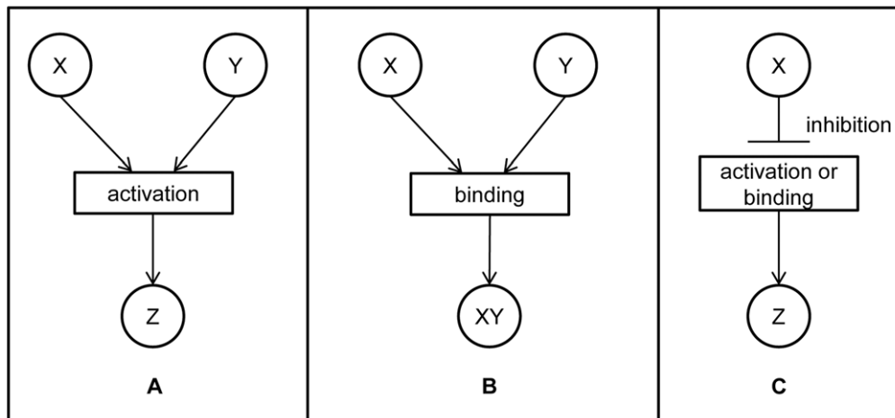
Figure 2. PDS reaction types. There are three groups of reactions. A) Activation (A) denotes all the reactions directly involving two components X and Y in the production of Z, where the concentration Z depends on the concentration of both substrates. B) Binding (B) results in the formation of a protein-protein complex or in the binding of a protein to a DNA promoter region to regulate its gene expression. C) Inhibition (I) is a process in which one component blocks the performance of another component. doi:10.1371/journal.pone.0051822.g002
