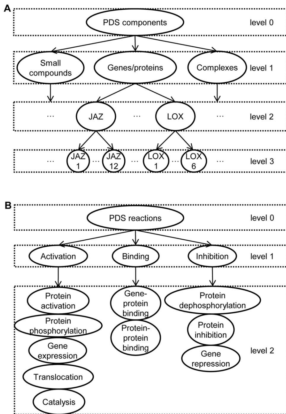
Figure 1. Taxonomy of PDS components and reactions. A) In the taxonomy of PDS components there are four representation levels. The highest level (level 0) is the most abstract level, while the lowest one (level 3) represents single molecules. B) In the taxonomy of PDS reactions individual reactions are represented at the lowest level (level 2) and are grouped according to their functionality into three groups at level 1: Activation (A) , Binding (B) and Inhibition (I) . doi:10.1371/journal.pone.0051822.g001
