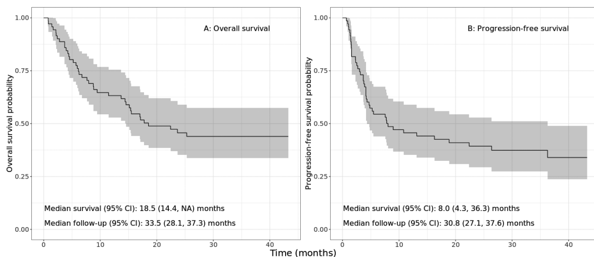
FIGURE 1. Kaplan-Meier curves show overall survival (OS) probability ( A ) and progression-free survival (PFS) probability ( B ) over time in patients with metastatic melanoma treated with immune checkpoint inhibitors. The grey shading reflects the 95% confidence interval.
