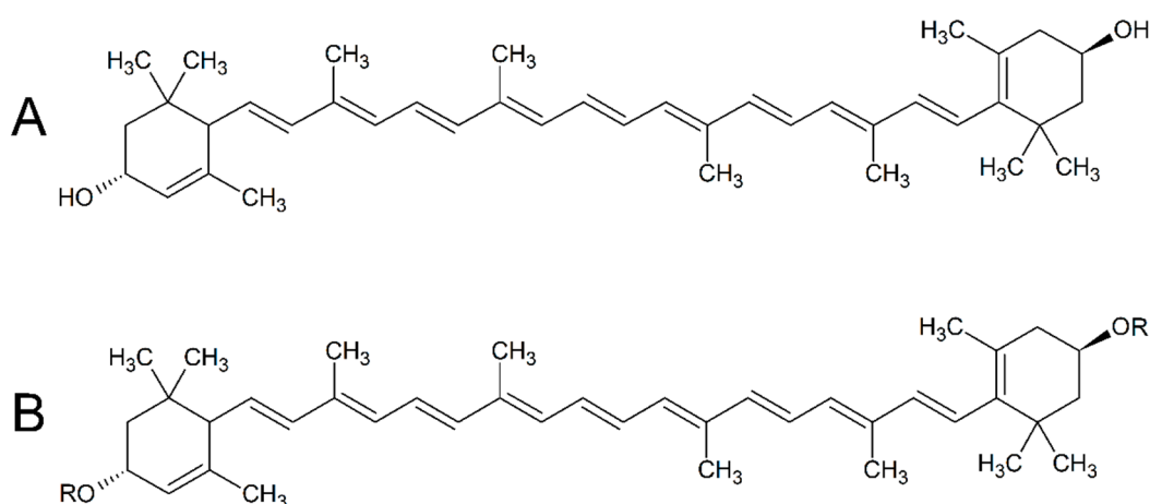
Figure 1. Structural formulae of lutein (A) and lutein esters (B) (common examples: R = palmitate, myristate, linoleate, laurate).
