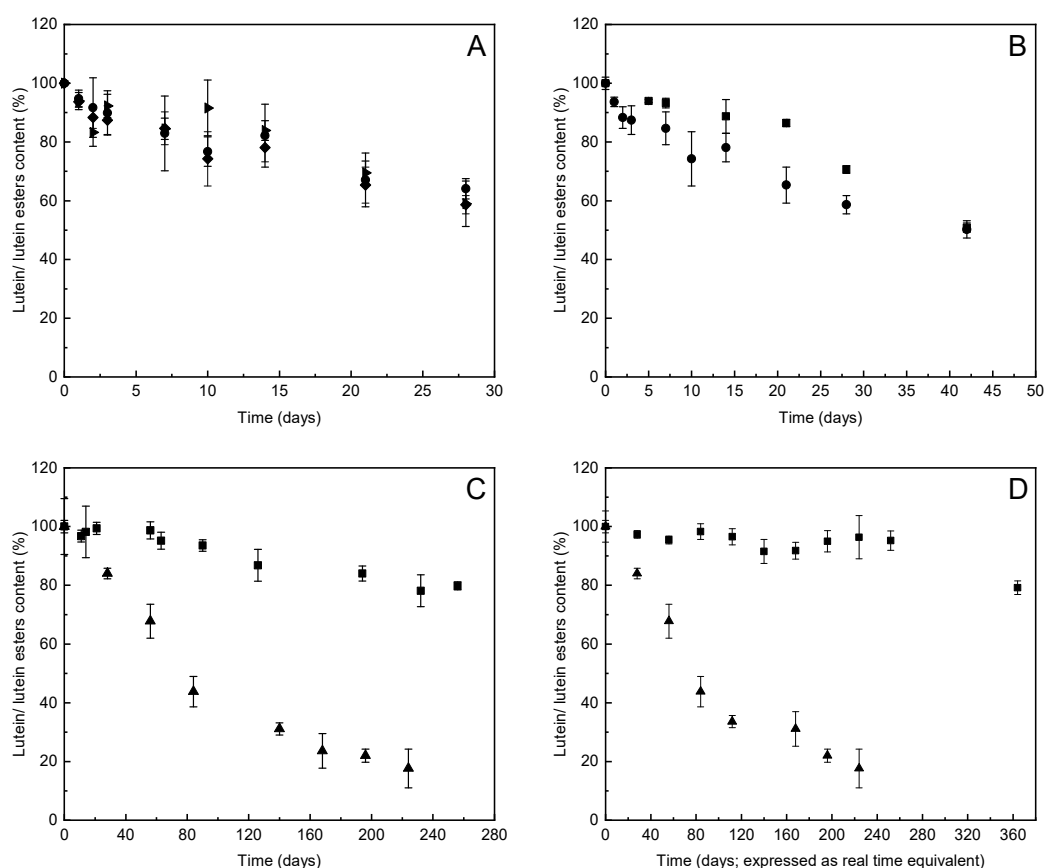
Figure 3. (A) Stabilities of formulation 3L (viscous emulsion) with lutein extract over 30 days under different storage conditions: In the light at 25 °C (▴); in the dark at 25 °C (◆); and in the dark at 4 °C (●). (B) Stabilities of formulation 3L (viscous emulsion) with lutein over 42 days at 25 °C in the dark without (●) and with (■) vitamin E. (C,D) Long-term stabilities of formulations 3L with lutein (▲) and 3LE with lutein esters (■) following real time at 25 °C in the dark (C) and accelerated conditions of storage at 37 °C in the dark (D). Time scale is calculated to real time. Data are means \pm SD ( n = 3 ).
