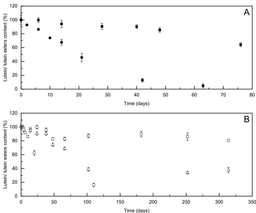
Figure 2. (A) Stabilities of lutein extract (●) and lutein esters extract (■) when stored in sealed dark containers at 4 °C. (B) Stabilities of formulation 2L with lutein (fine suspension, ○) and formulations 1LE (paste, △) and 2LE (fine suspension, □) with lutein esters when stored in sealed dark containers at 25 °C. Data are means \pm SD ( n = 3 ).
