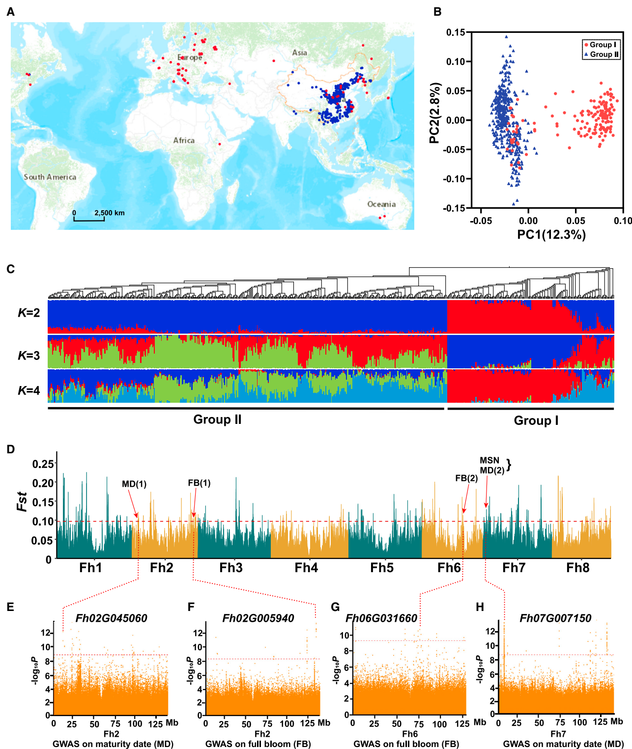
Figure 4. Population feature and divergence of common buckwheat
