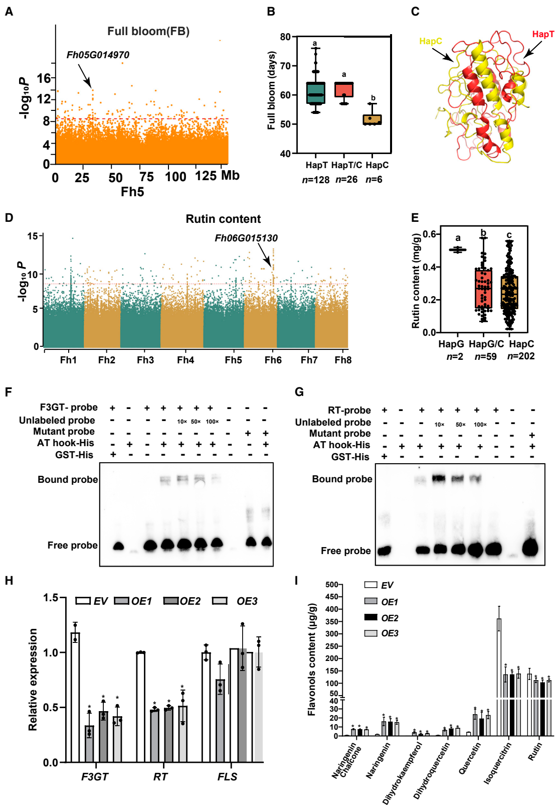
Figure 5. Identification of genes associated with agronomic traits of buckwheat (A) Manhattan plot for GWAS association with full bloom (FB, days). The dashed line indicates the threshold -\log P = 8.5 . The black arrow indicates the SNP in Fh05G014970 .
