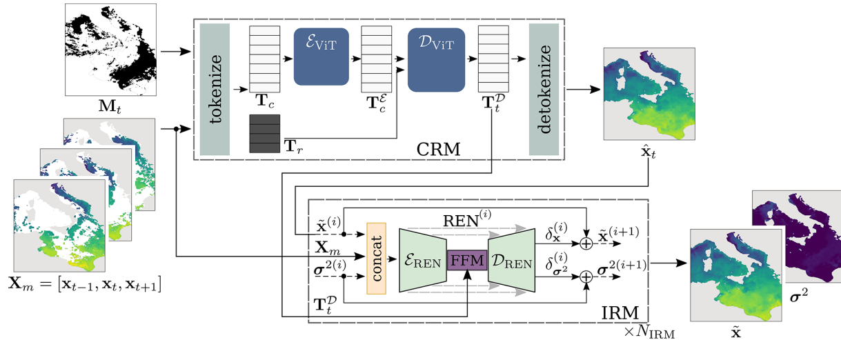
Figure 2. Given observations for 3 consecutive days [x_{t-1}, x_t, x_{t+1}] and a binary mask \mathbf{M}_t indicating missing pixels, CRITER densely reconstructs x_t in two phases. First, the CRM estimates a coarse reconstruction \hat{x}_t , which the IRM then iteratively refines to produce the final reconstruction \tilde{x} and uncertainty \sigma^2 . CRM tokenizes the input into tokens requiring reconstruction \mathbf{T}_r and contextual tokens \mathbf{T}_c . These contextual tokens are encoded by a ViT-based encoder into \mathbf{T}_c^E , combined with \mathbf{T}_r , and decoded by a ViT-based decoder into decoded tokens \mathbf{T}_t^D , which are finally mapped to \hat{x}_t . In the IRM, dashed lines indicate the iterative refinement process. At each iteration i , the current reconstruction estimate \tilde{x}^{(i)} and uncertainty estimate \sigma^{2(i)} are refined by adding the predicted residuals: reconstruction residual \delta_x^{(i)} and uncertainty residual \delta_{\sigma^2}^{(i)} . The index in \text{REN}^{(i)} indicates the change in network parameters in each iteration.
