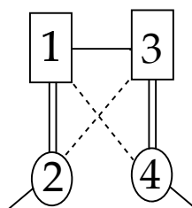
Figure 4: A symmetry-type graph (in fact, a diagram as defined in 8.1) of a map with respect to a group of symmetries acting on a wedge corneration. The 0-edges are depicted with dotted lines, 1-edges with single solid lines and 2-edges with double solid lines. Boxed vertices 1 and 3 correspond to orbits of in-wedges while the ovals 2 and 4 correspond to orbits of out-wedges.
