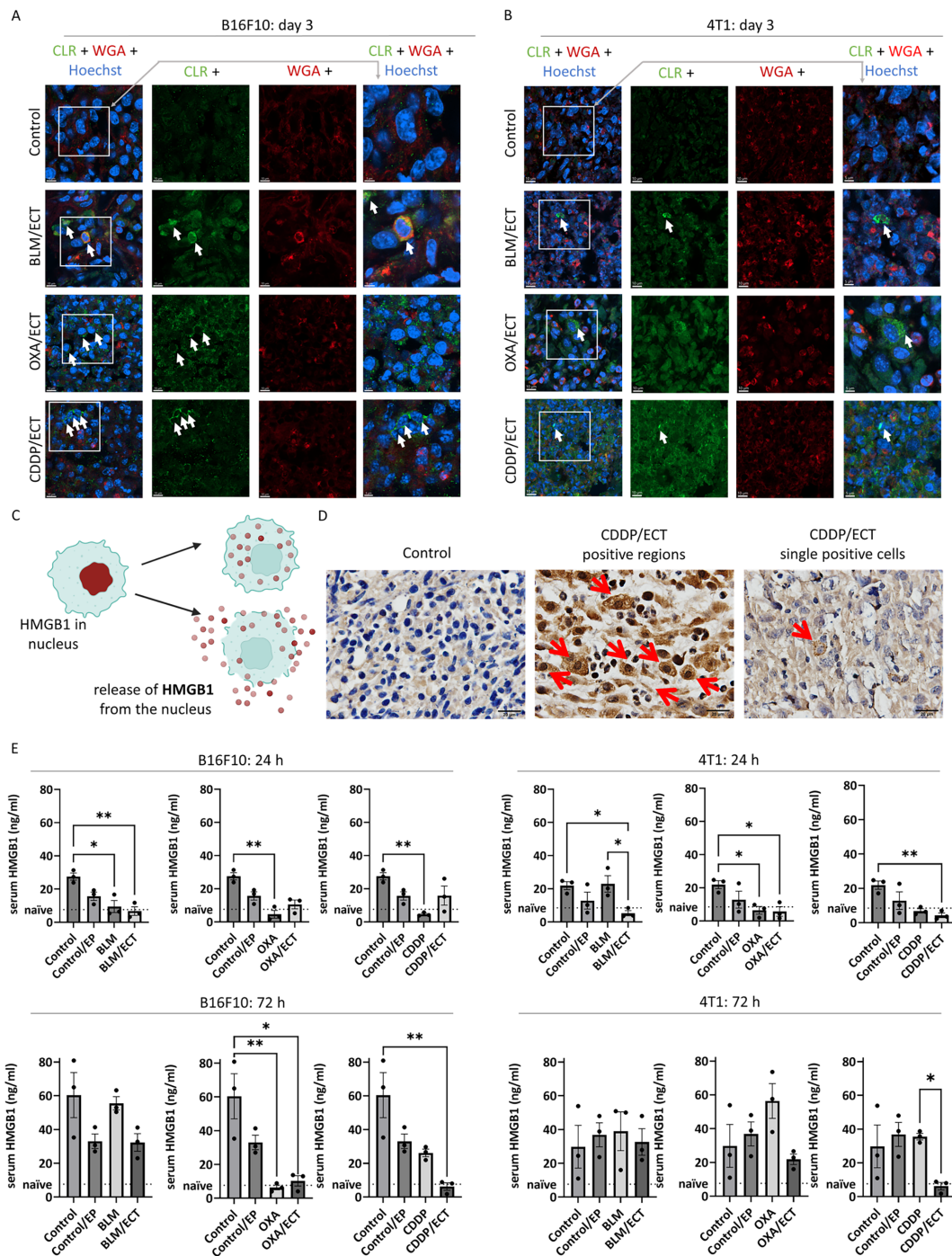
FIGURE 4 Immunogenic cell death is induced after ECT. Two markers of immunogenic cell death were investigated; calreticulin (CLR) exposure to plasma membrane and high-mobility group box 1 (HMGB1) protein release from dying cells. CLR was exposed to plasma membrane after ECT with BLM, OXA or CDDP in (A) B16F10 and (B) 4T1 tumors. Arrows indicate colocalization of CLR (green) and membranes (WGA, red). Scale bar: 10 \mu m (column 1-3) or 5 \mu m (column 4). (C) During immunogenic cell death, HMGB1 is released from nucleus as presented in the drawing. (D) Representative microphotographies of HMGB1 positive 4T1 tumor regions as well as single tumor cells releasing HMGB1. Arrows indicate IHC positive signal. Scale bar: 20 \mu m. (E) Serum concentration of HMGB1 24 and 72 hours after the treatment in mice bearing B16F10 and 4T1 tumors. (n = 3; AM \pm SE and individual measurements are presented *p \leq 0.05, **p \leq 0.01).
