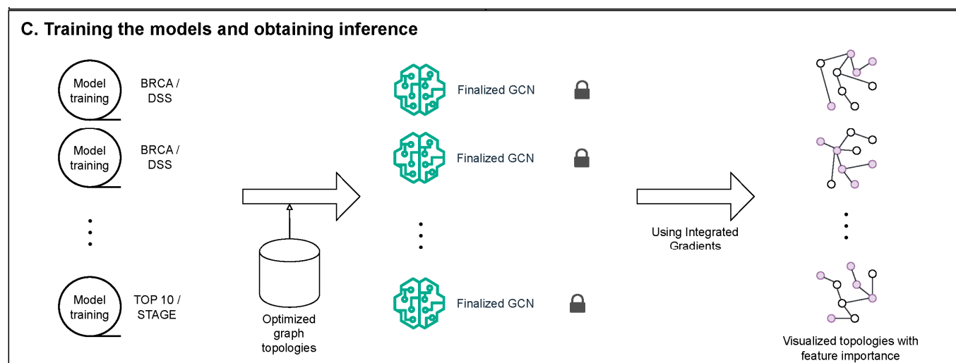
Figure 1. Study overview. (A) Projecting gene expression data across cancer cohorts as graphs. (B) Heuristic search using the genetic algorithm optimization technique for each use case. (C) Training the models and visualizing inference by highlighting the most important gene activations in the pathway.
