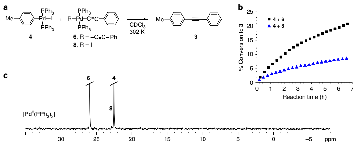
Fig. 4 Probing transmetallation. a Reaction between 4 (1.0 equiv., 0.013 M) and acetylide 8 or 6 (1.2 equiv., 0.016 M). b Tolane 3 build-up. c 31 P NMR analysis of the reaction mixture between 4 and 6 incubated for 90 min (Supplementary Note 3 and Supplementary Figs. 15–16)
