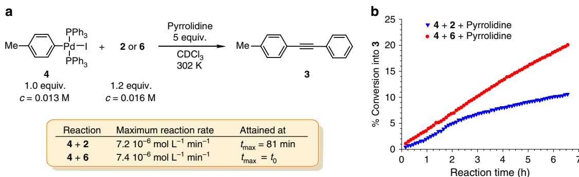
Fig. 5 Putting on trial the mono-metallic mechanism from Fig. 1c. a Independent reaction between authentic 4 and 6 or acetylene 2 in the presence of pyrrolidine. b Tolun 3 build-up (Supplementary Note 3 and Supplementary Figs. 17–22)
