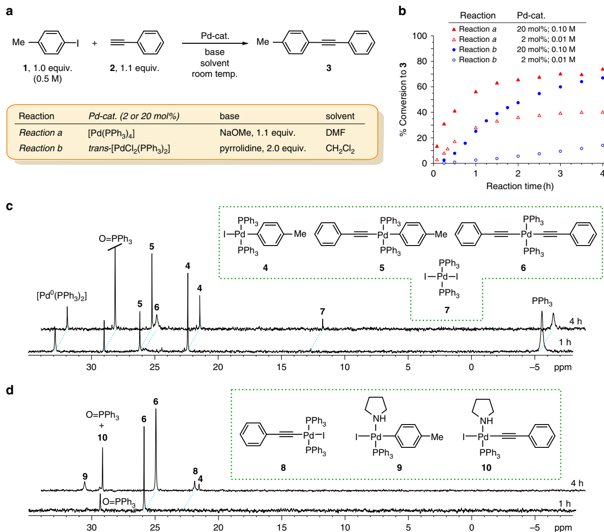
Fig. 2 Model reactions and conditions with the proposed phosphorous containing species. a , b Reaction conditions ( a ) and product 3 build-up as determined by ^1\text{H} NMR spectroscopy ( b ). c ^{31}\text{P} NMR spectra of aliquots from Reaction a (with 20 mol% of Pd-cat.), after 1 and 4 h. d ^{31}\text{P} NMR spectra of aliquots from Reaction b (with 20 mol% of Pd-cat.), after 1 and 4 h. Relative intensities of the resonances do not correspond to the concentrations of the species. For spectra showing more frequent sampling, see Supplementary Figs. 1–8
