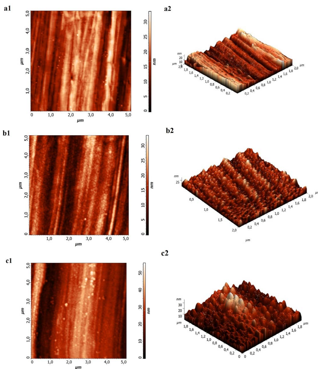
Figure 6: Surface topography on 5 \times 5 \mu\text{m} (2D) and on 2 \times 2 \mu\text{m} area (3D) for a) untreated PP tube, b) PP 5x plasma treated tube, and c) PP 20x plasma treated tube.
