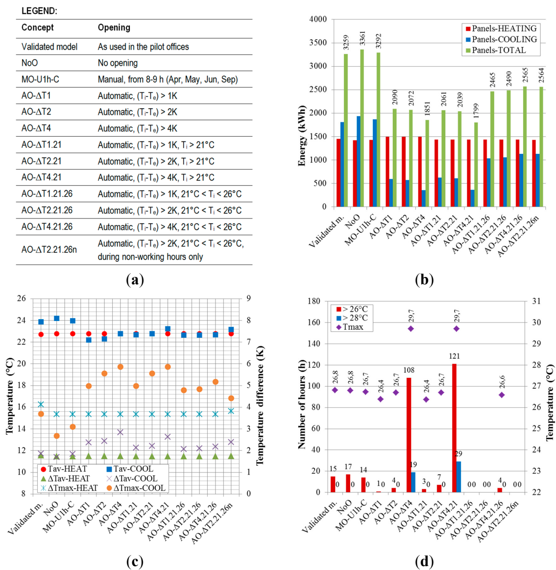
Figure 10. (a) Legend for graphs; (b) The simulated energy of the whole model; (c) the simulated air temperatures in Office 2; and (d) the hours when the air temperature limits were exceeded in Office 2, for different window opening strategies (note: glazing and shading were not changed).
