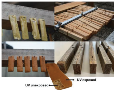
Figure 1: Weathering of PUR adhesive in Slovenia and lap shear test specimens.
