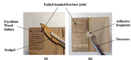
Figure 5: Preparation of FTIR adhesive specimens in New Zealand (a) Wood substrate cut adjacent to bond line (b) Extraction of adhesive fragment.
