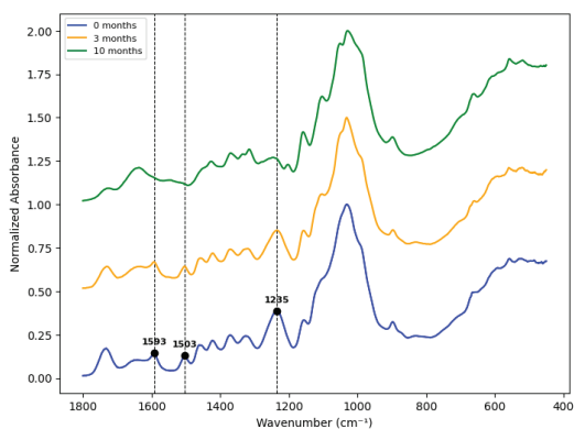
Figure 10: FTIR spectra of beech wood surface during 3 and 10 months of full weather exposure.
