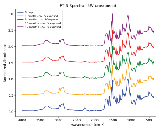
Figure 11: FTIR spectra of full weather unexposed part of adhesive, during 1, 3, 10 and 12 months of natural ageing.
