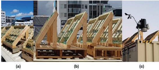
Figure 2: Natural weathering arrangements in New Zealand (a) Weather rack angle view (b) Weather rack side view (c) Elevated weather station.
