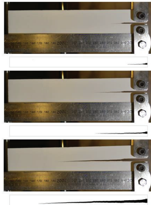
Figure 4: Crack length propagation and determination during Mode I testing in New Zealand.
