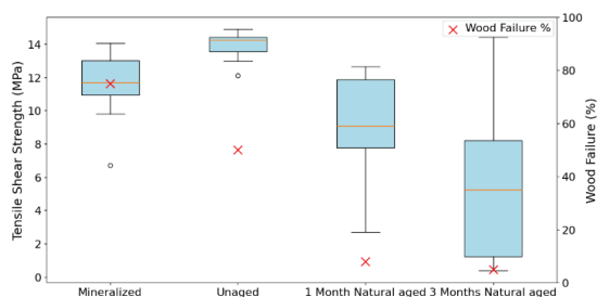
Figure 7: Results of lap shear test of mineralized bonded beech wood and native bonded beech wood specimens after 1 and 3 months of full weather exposure.
