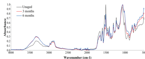
Figure 8: Representative FTIR spectra of PUR 2 bonded CCA preservative-treated samples.
