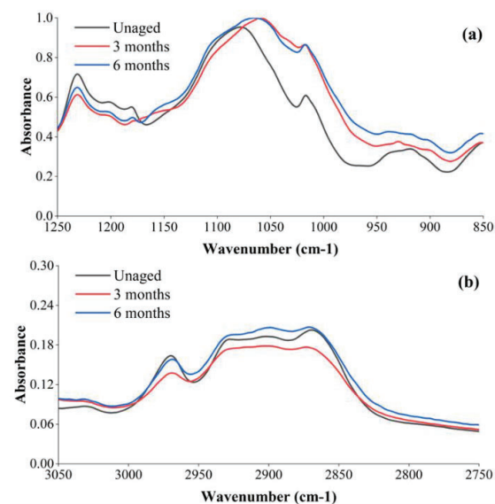
Figure 9: FTIR spectra of PUR 2 bonded CCA preservative-treated samples after constant long-term high temperature and humidity ageing (a) 850\text{--}1250\text{ cm}^{-1} (C–O) region (b) 2750\text{--}3050\text{ cm}^{-1} (C–H) region.
