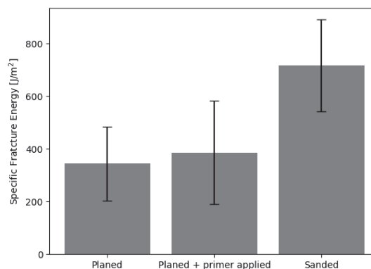
Figure 6: Specific fracture energy results of bonded beech wood with different surface preparation methods prior adhesive bonding.
