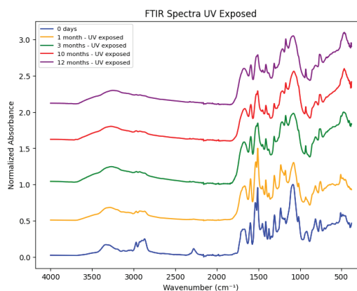
Figure 12: FTIR spectra of full weather exposed part of adhesive, during 1, 3, 10 and 12 months of natural ageing.
