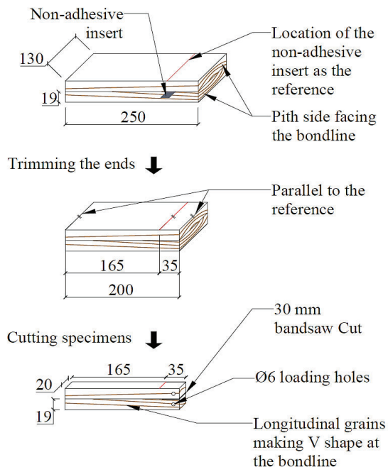
Figure 3: Manufacture of Mode I glued laminated wood specimens in New Zealand. Dimensions are given in mm.
