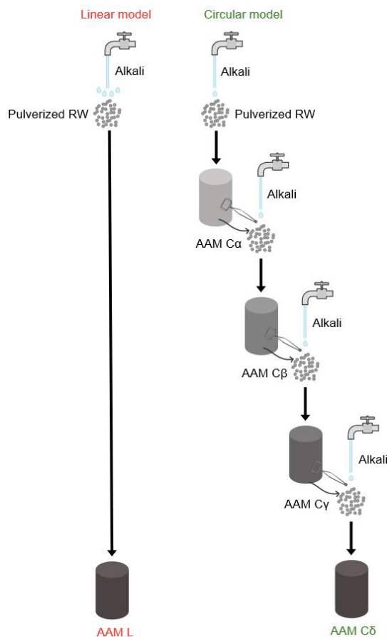
Figure 1: Synthesis scheme.
