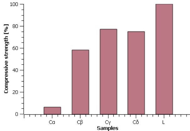
Figure 3: Compressive strength normalised to the compressive strength of the sample from the linear model.
