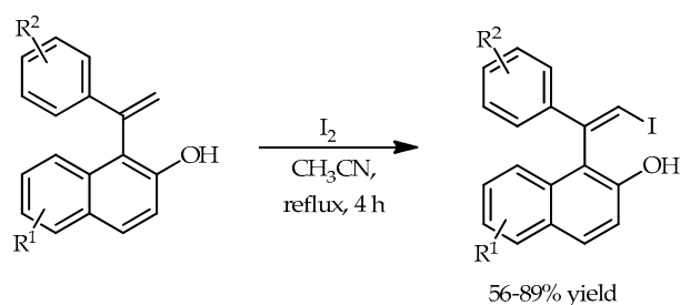
Scheme 22. Vinyl iodination of ortho -vinylnaphthols with I_2 .
