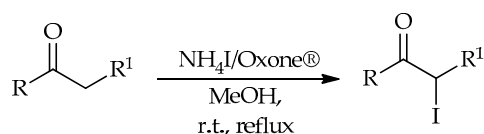
Scheme 53. \alpha -Iodination of alkyl ketones using \text{NH}_4\text{I} /oxone ® system.
