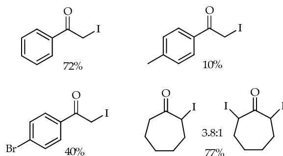
Scheme 55. Synthesis of \alpha -iodo alkyl ketones using \text{NH}_4\text{I}/\text{oxone}^\circledast system.
