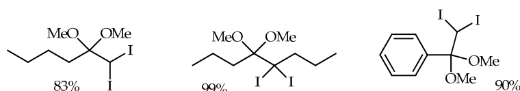
Scheme 11. Diiododimethoxylation of alkynes.
