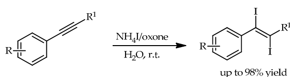
Scheme 35. Oxidative ( E )-diiodination of alkynes using NH 4 I/oxone system.
