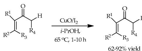
Scheme 47. Iodination of \alpha,\beta -unsaturated ketones using CuO/I_2 .
