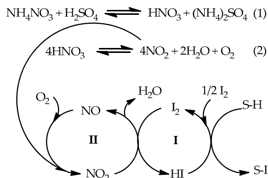
Scheme 51. The reaction pathway for the aerobic oxidative \alpha -iodination employing air/ \text{NH}_4\text{NO}_3 (cat.)/ \text{I}_2/\text{H}_2\text{SO}_4 (cat.).
