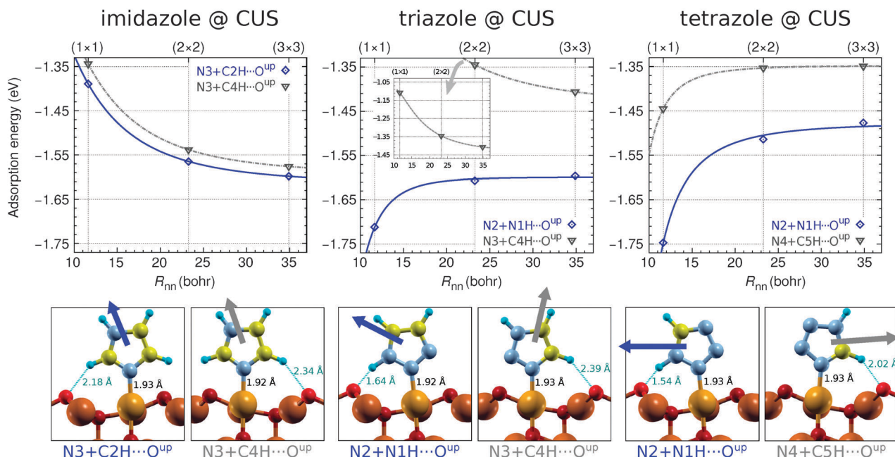
Fig. 2 As in Fig. 1 but for the molecular bonding at a CUS site. Adsorption energies are calculated with respect to the high-symmetry position of Cu CUS ions in the bare substrate to better represent the molecule–surface bond strengths. Note that the Cu CUS ions of the bare substrate relax laterally to a more stable asymmetric position if the symmetry is broken (see Fig. 1 in ref. 9) with an energy stabilization of 0.13 eV at full ( \theta = 1 ) and 0.04 eV at lower surface concentration ( \theta \leq 1/4 ) of extraneous Cu CUS ions at Cu 2 O(111)-w/o-Cu CUS .
